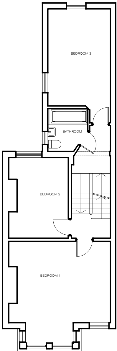
PROPOSED 1ST FLOOR SCALE 1:100
