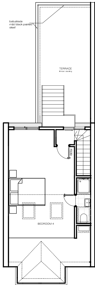
PROPOSED LOFT CONVERSION OPT1 SCALE 1:100
