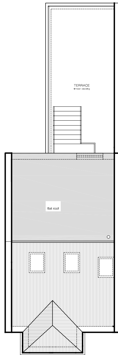
PROPOSED ROOFS SCALE 1:100
