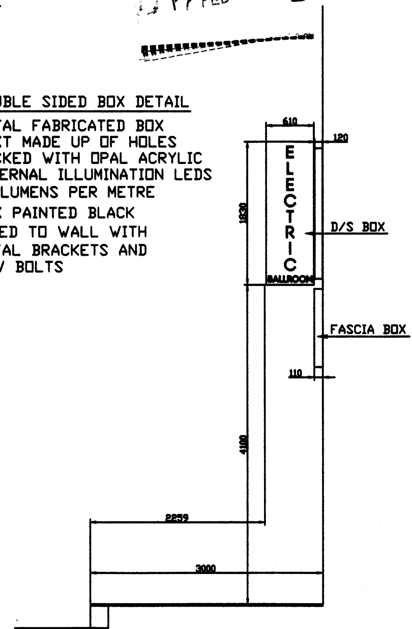
SIDE VIEW
