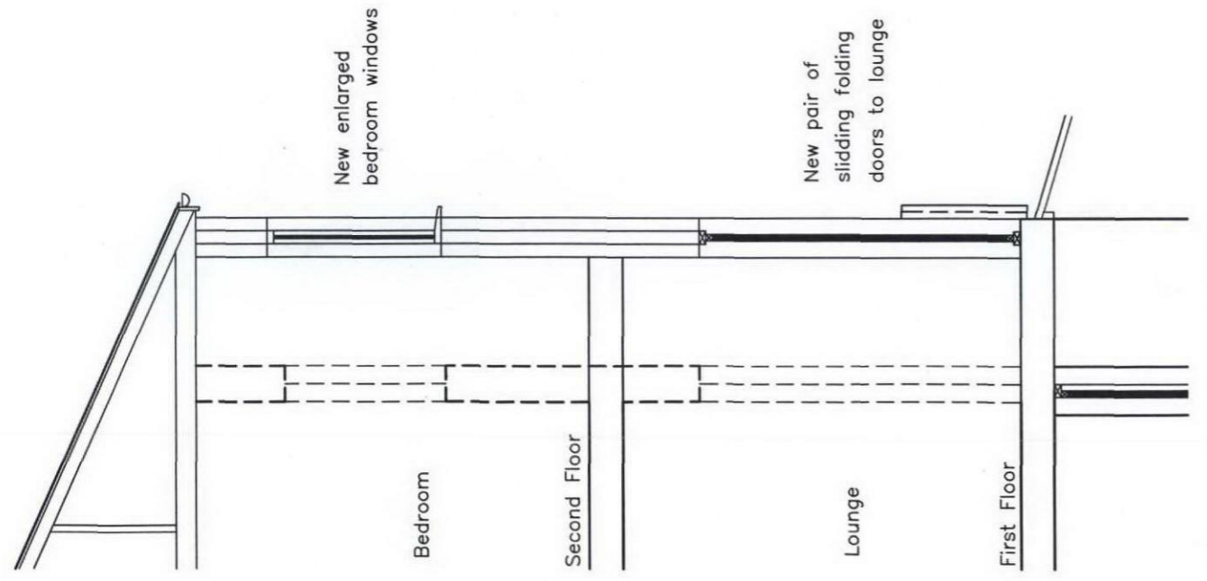
Section Thro' Door & Window
