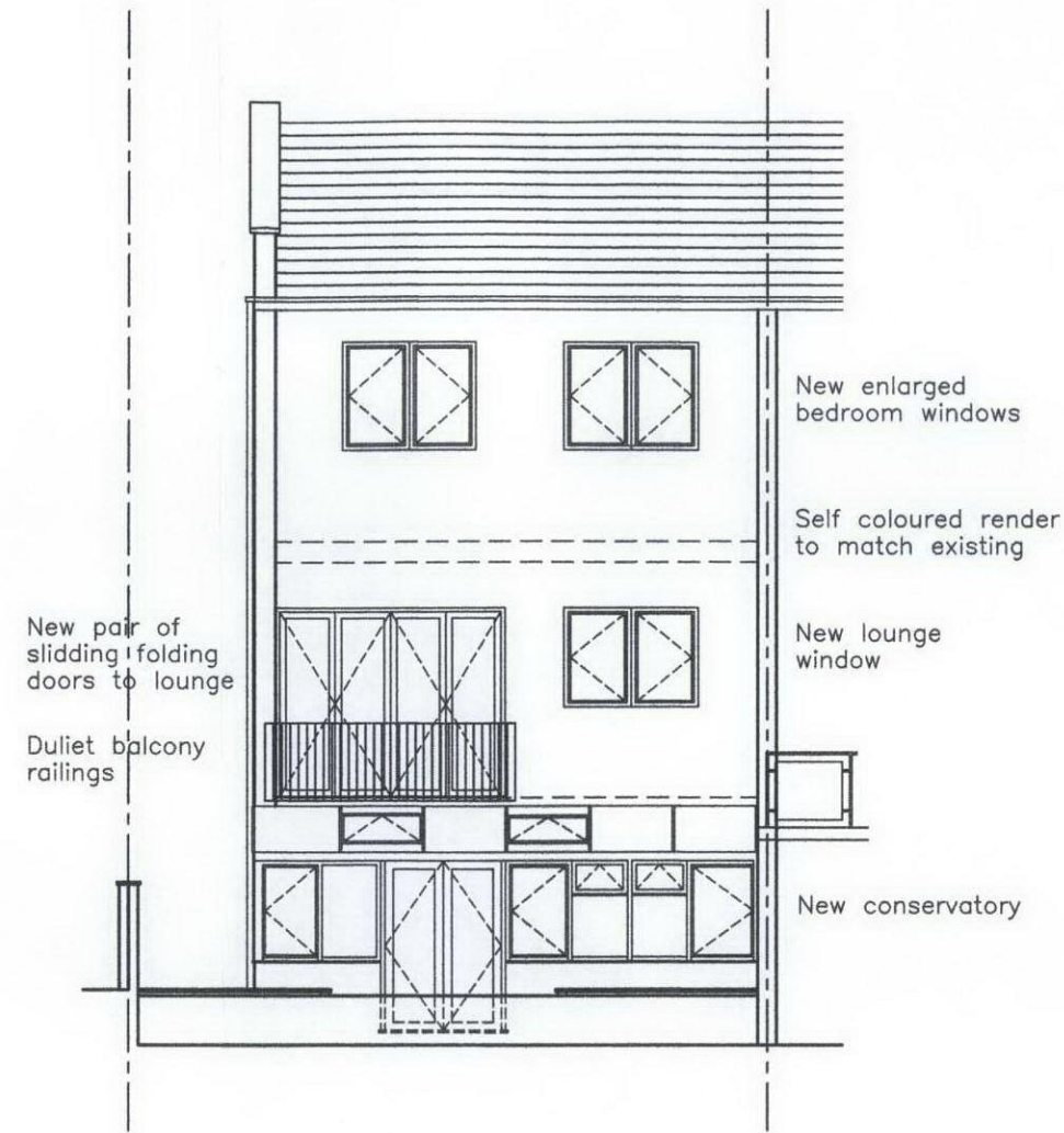
Rear Elevation
