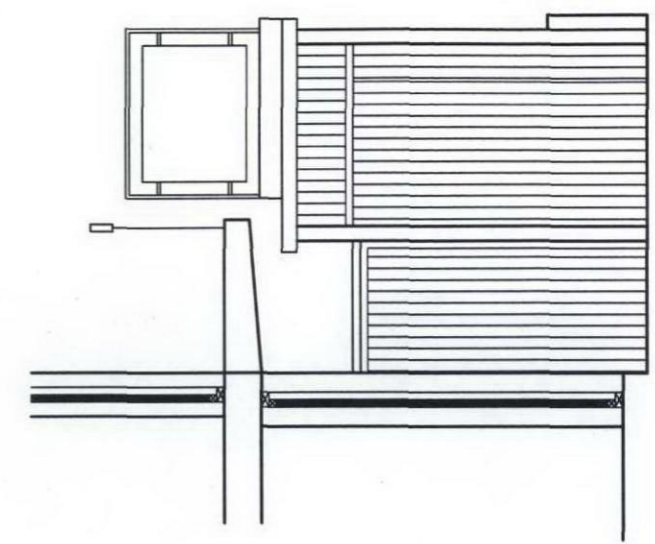
Section Thro' Conservatory & Existing Ground Floor Sliding Paton Doors
