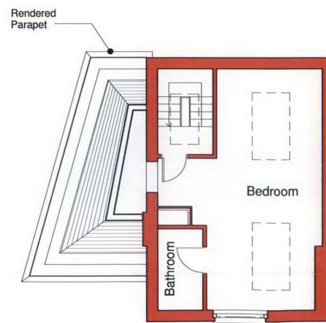
Third Floor
