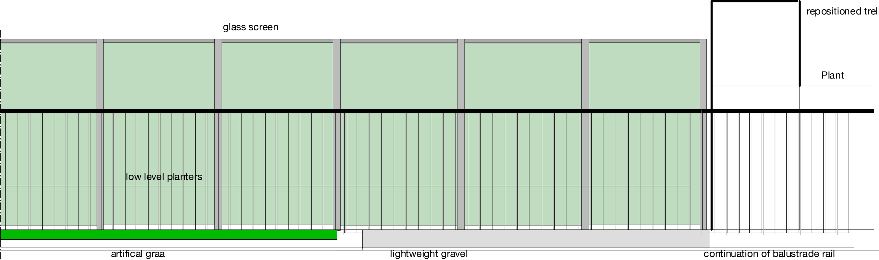
PROPOSED PART SIDE ELEVATION LOOKING FROM JOHNS STREET OF ROOF TERRACE SHOWING GLASS PANELS BB
