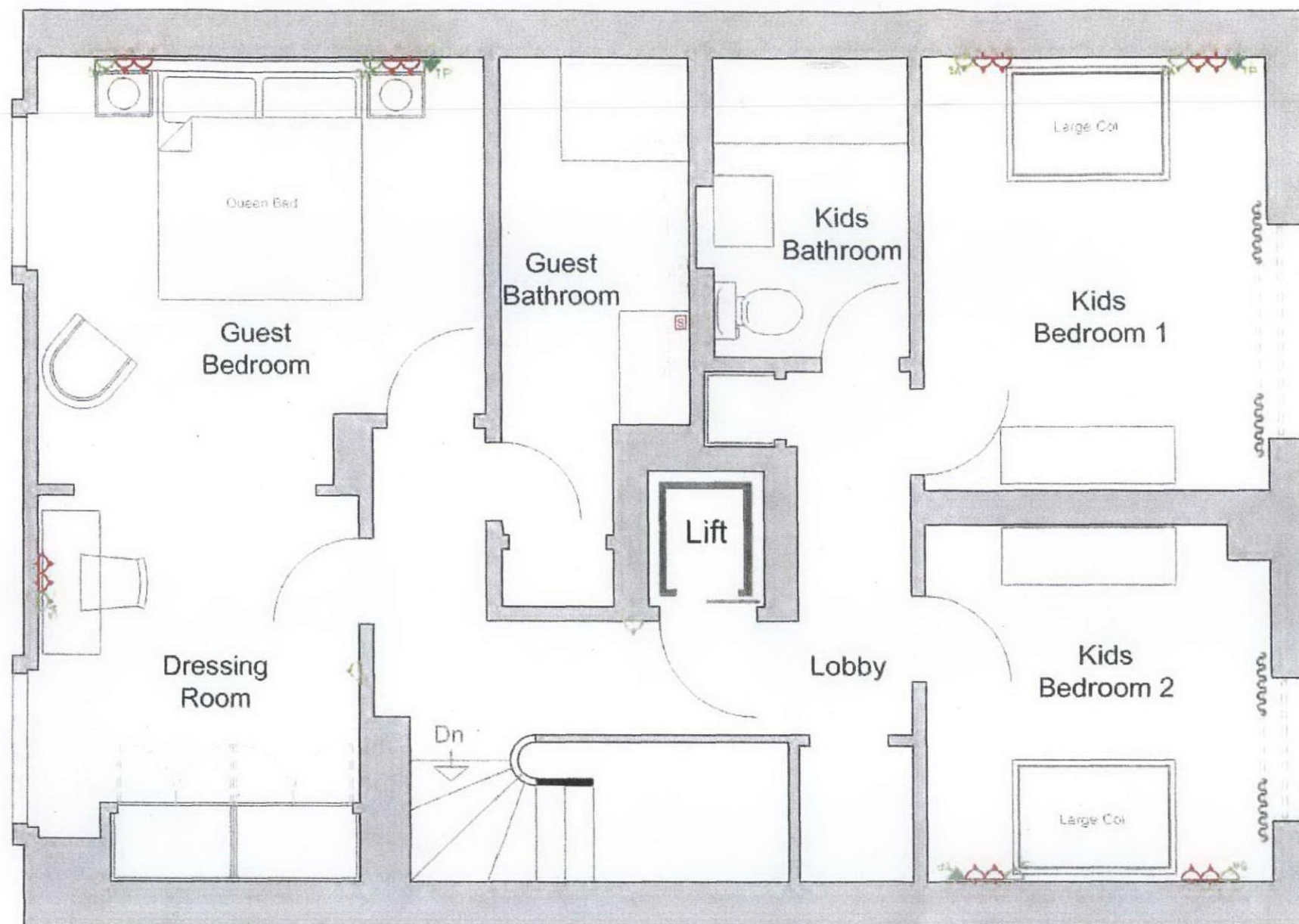
17 Chester Terrace - Proposed Small Power Plan Third Floor - 1:50@A3
