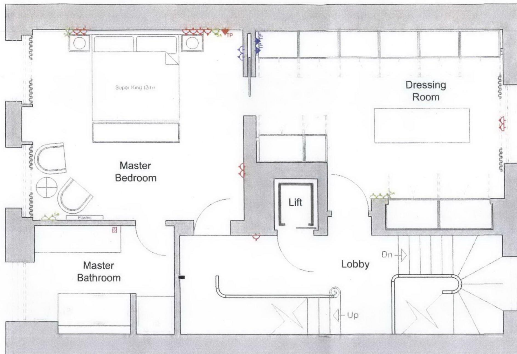
17 Chester Terrace - Proposed Small Power Plan Second Floor - 1:50@A3
