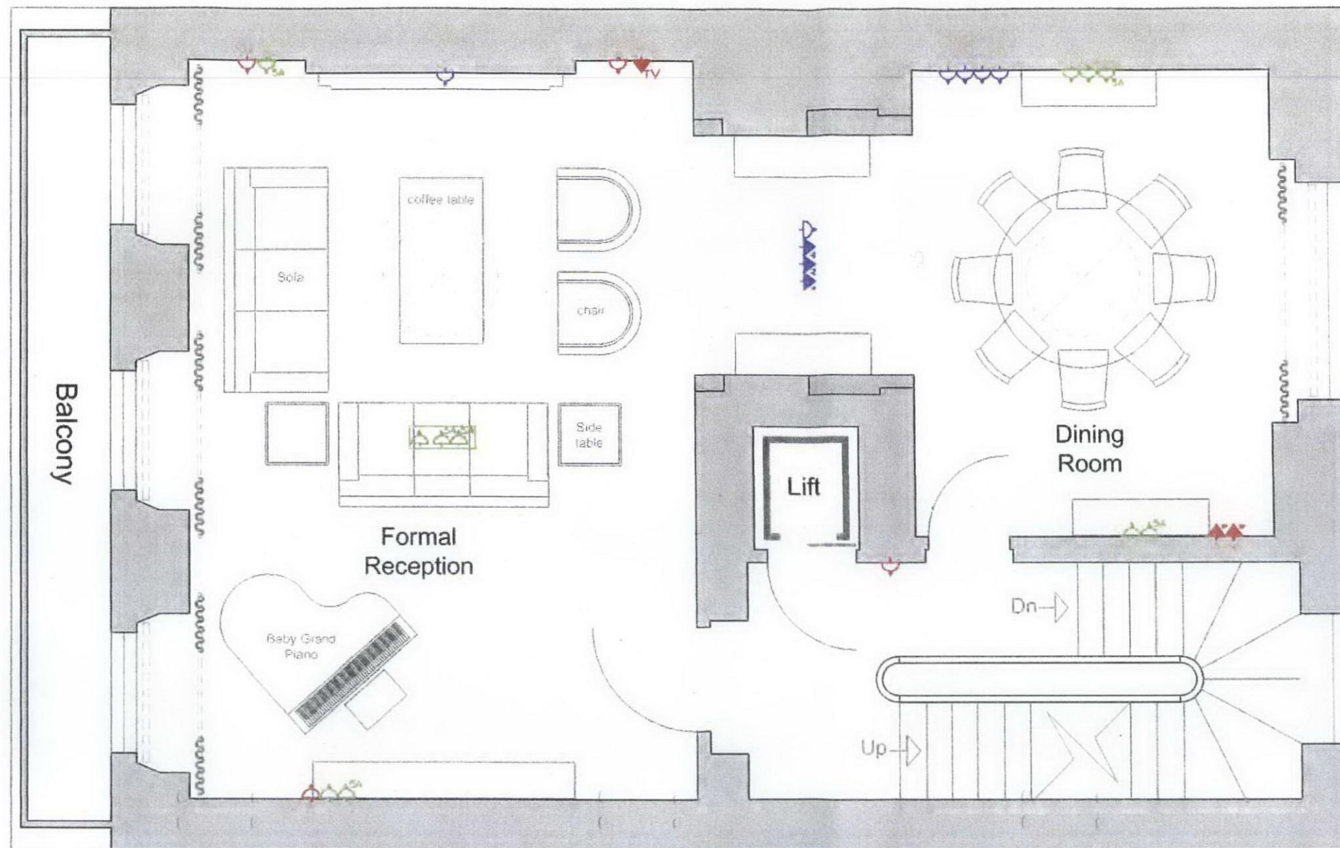
17 Chester Terrace - Proposed Small Power Plan FIRST FLOOR - 1:50@A3
