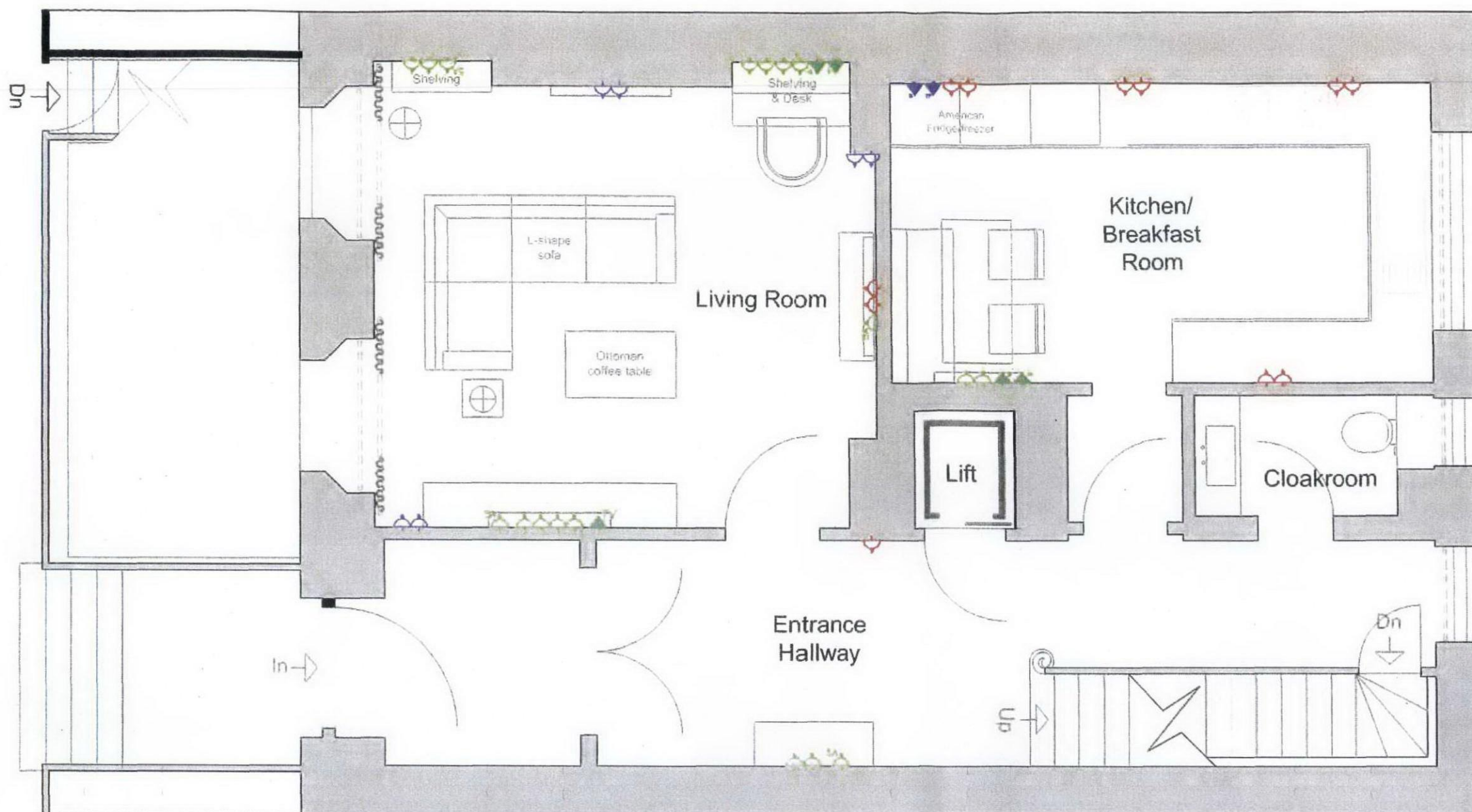
17 Chester Terrace - Proposed Small Power Plan Ground Floor - 1:50@A3
