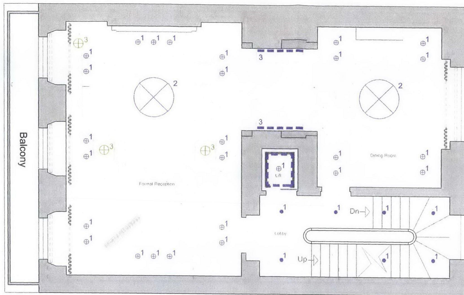
17 Chester Terrace - Proposed Lighting Layout First Floor - 1/50@A3
