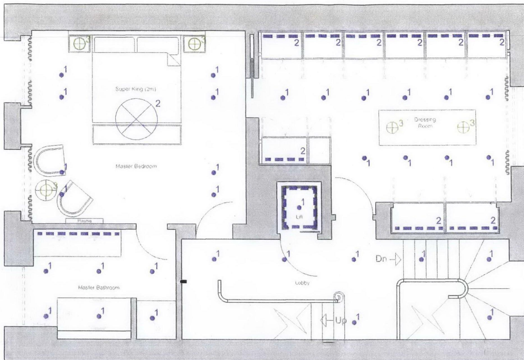
17 Chester Terrace - Proposed Lighting Layout Second Floor - 1/50@A3
