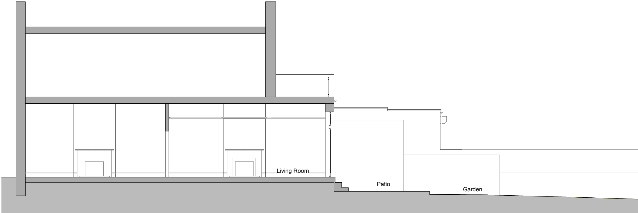
1 Existing Section A SE-003 scale 1:100 @ A4
