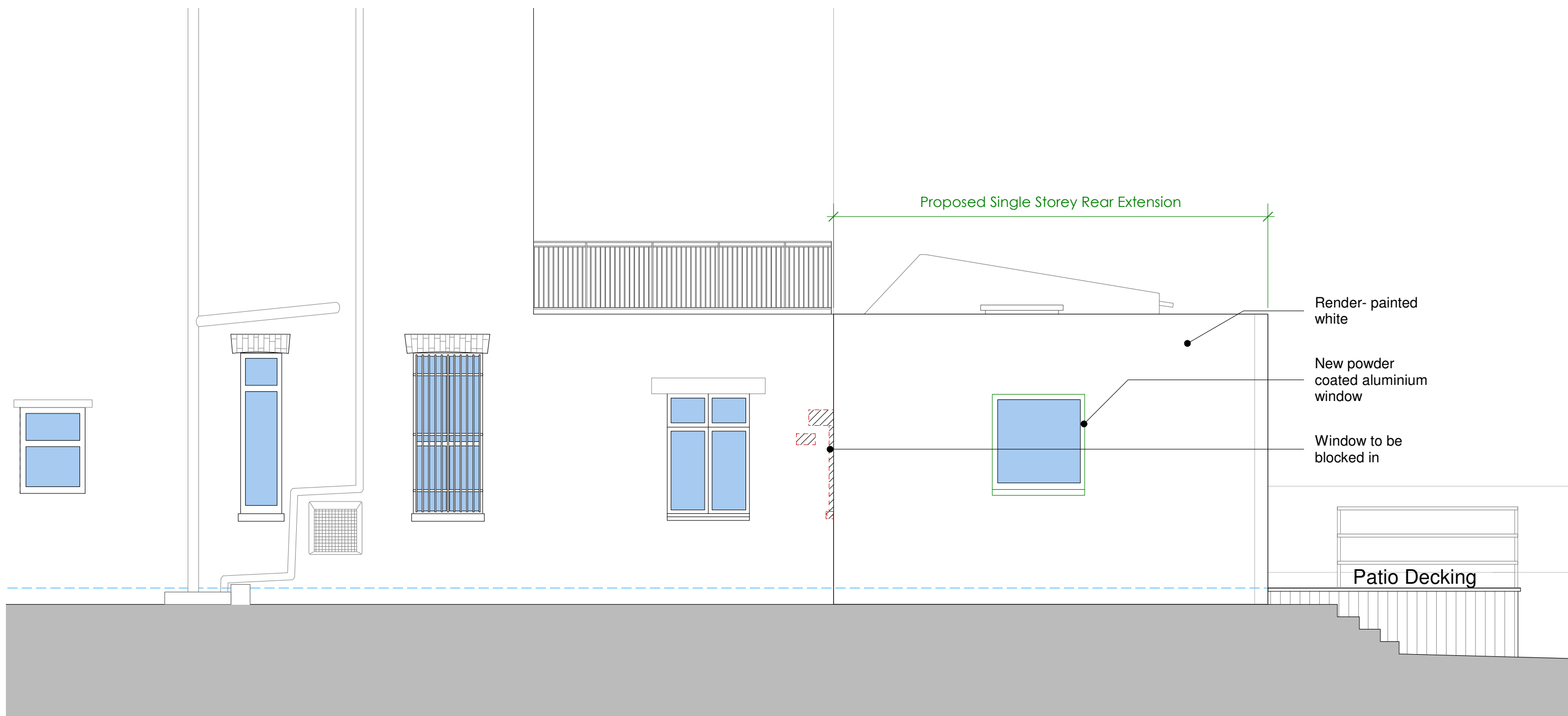
1 EL-013 Proposed West Elevation scale 1:50 @ A3
