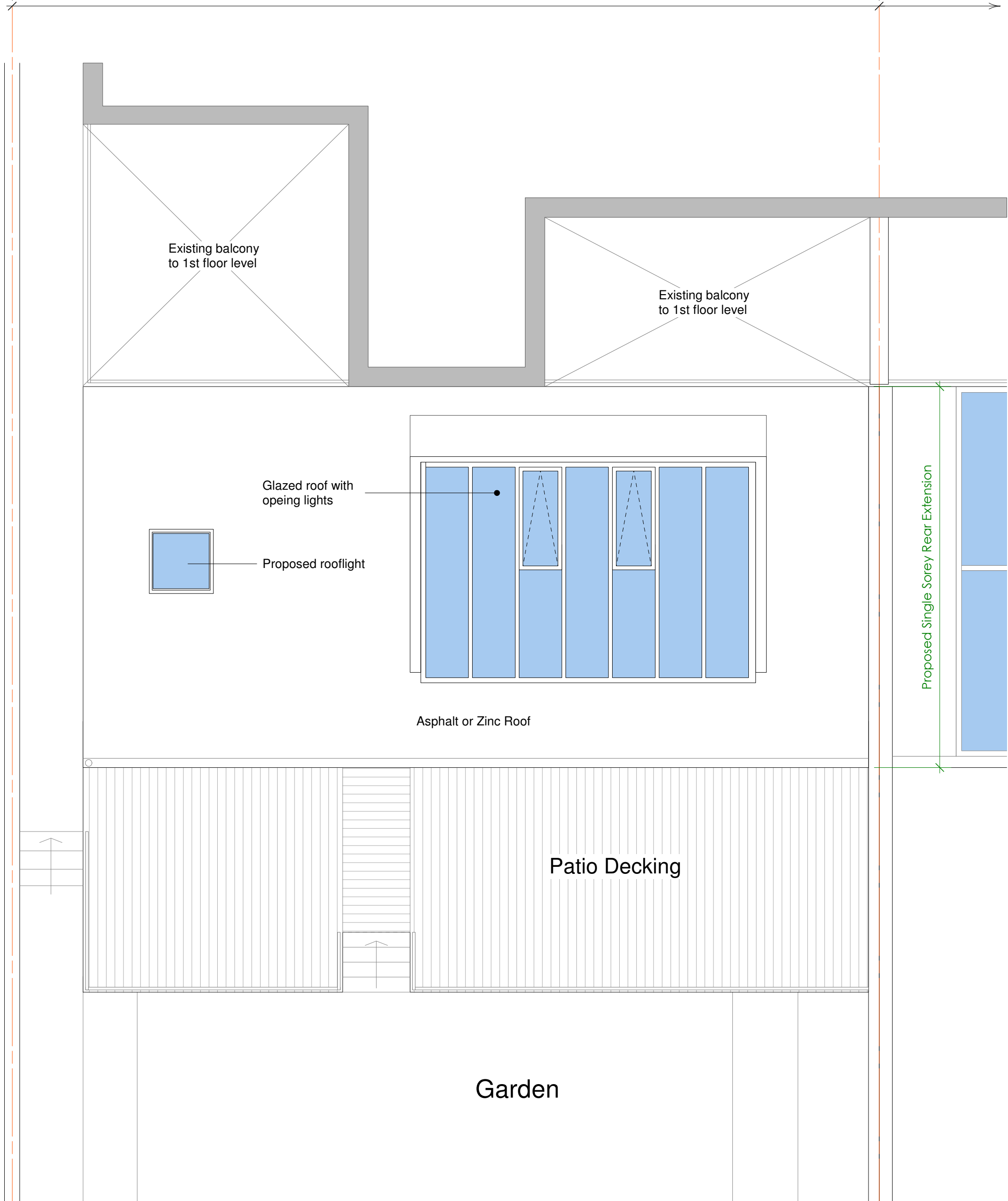
1 Proposed Roof Plan GA-019 scale 1:50 @ A3
