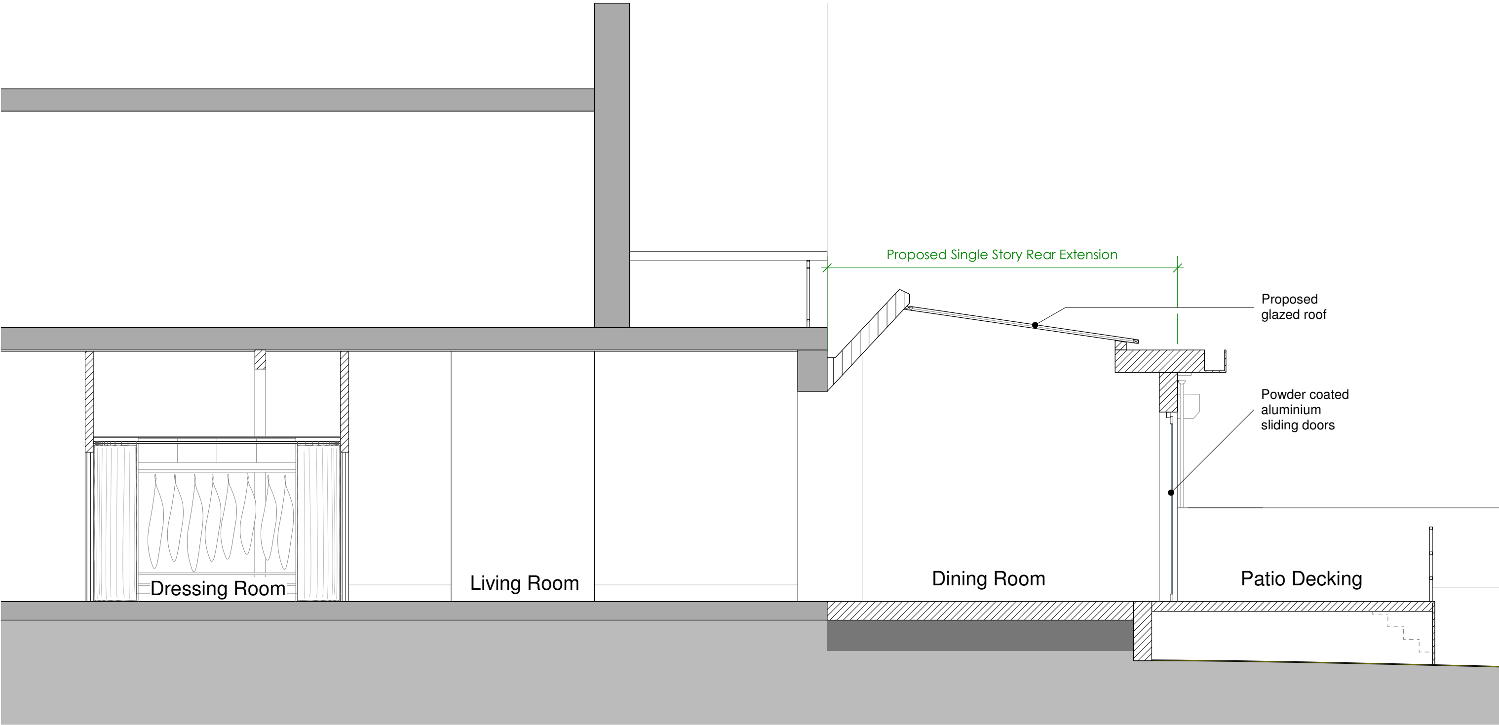
1 SE-017 Proposed Section A scale 1:50 @ A3
