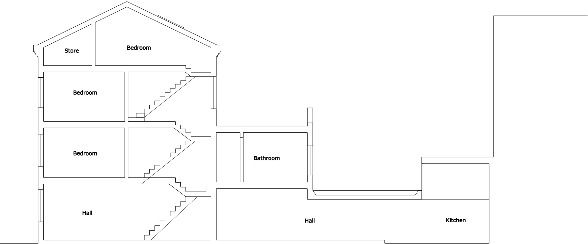
1 Long section as proposed AA 151_25 Scale 1:100 @ A3
