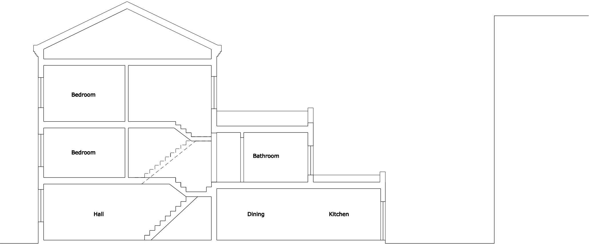
1 Long section as existing AA 151_15 Scale 1:100 @ A3
