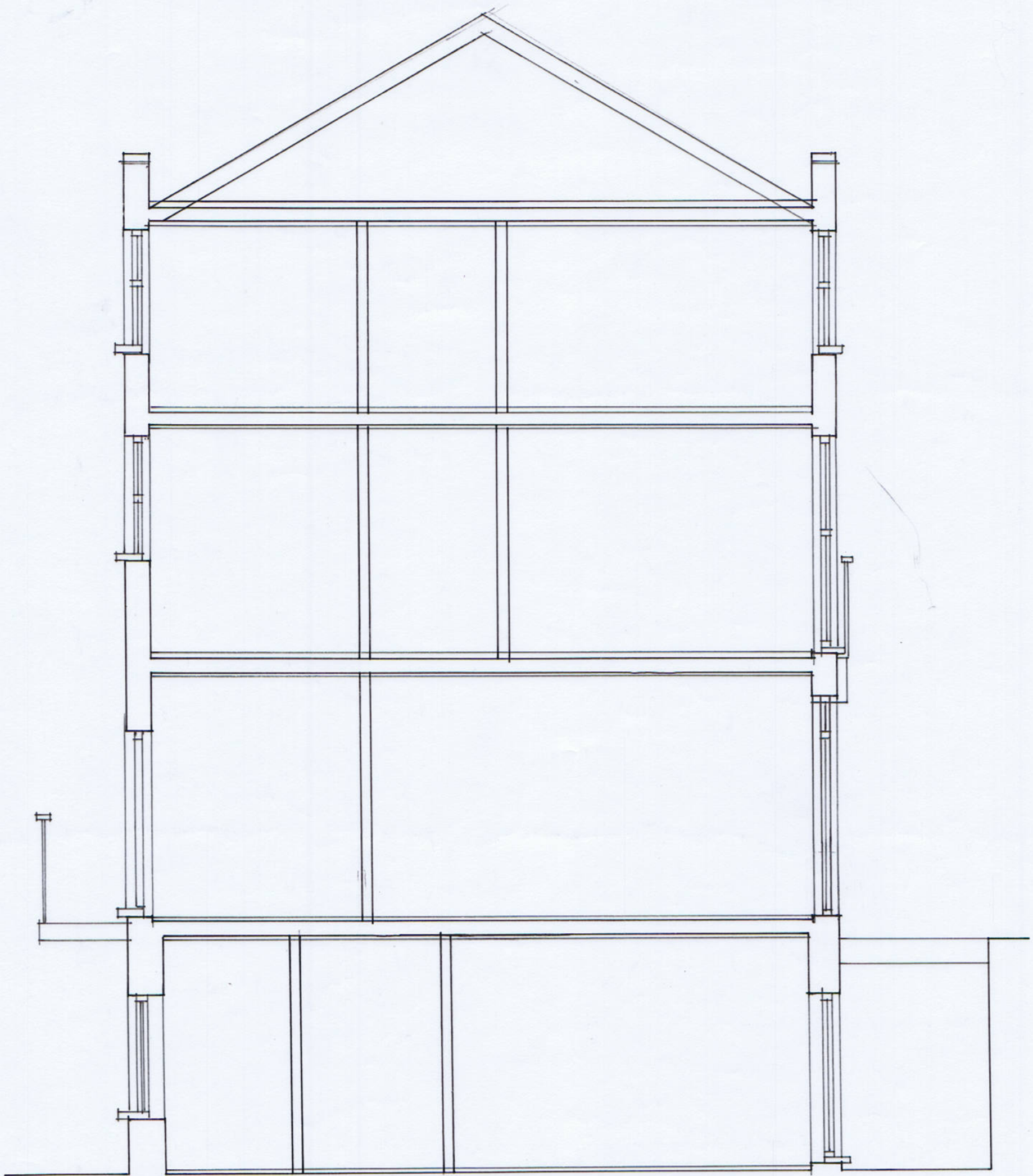
EXISTING LONGTIDUNAL SECTION A - A
