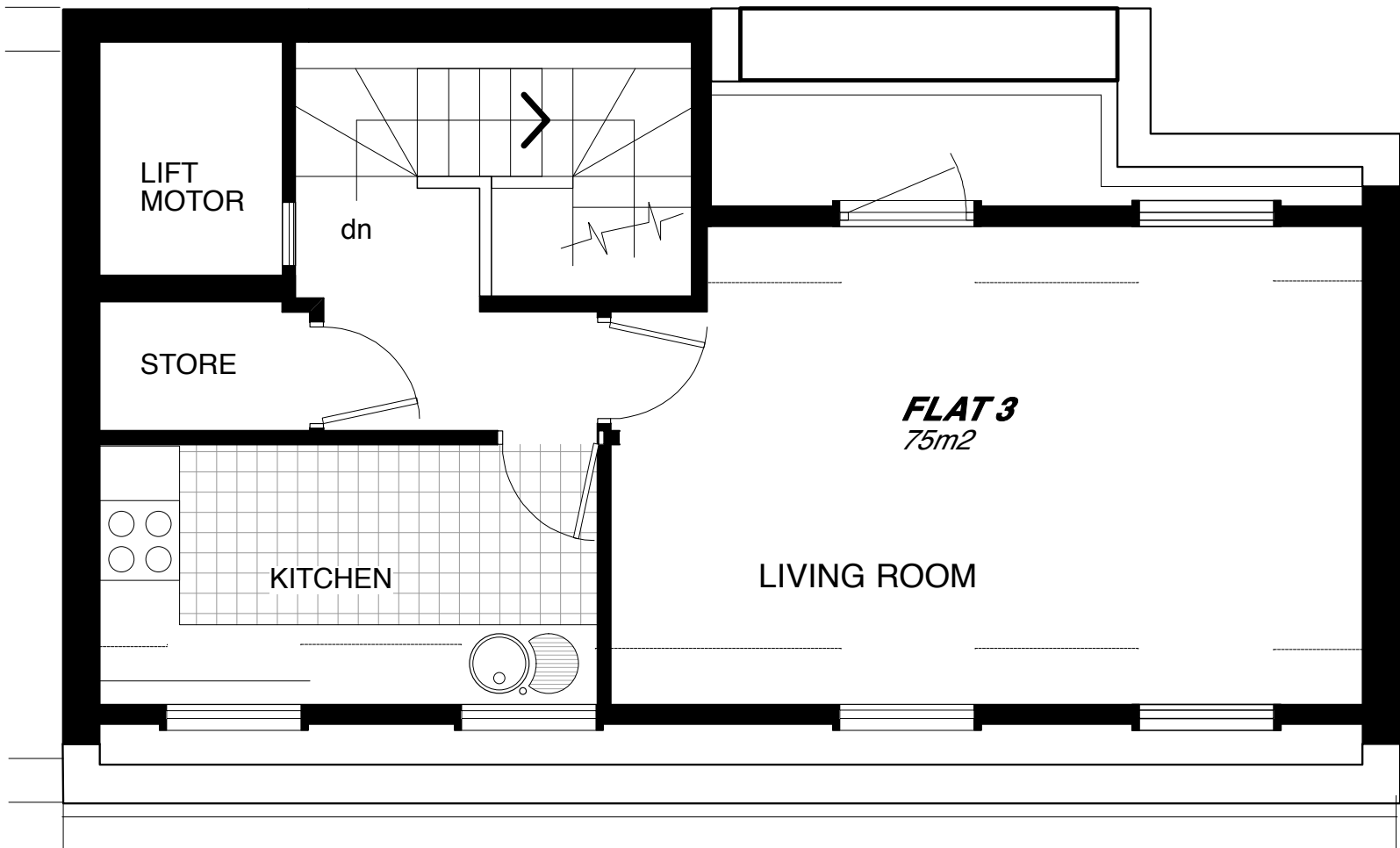
EXISTING 6th FLOOR PLAN scale 1:50
