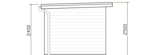
PROPOSED SUMMERHOUSE/STUDY NORTH-EAST ELEVATION 1:100
