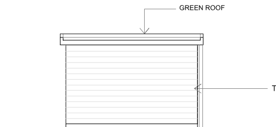
PROPOSED SUMMERHOUSE/STUDY SOUTH-EAST ELEVATION 1:100
