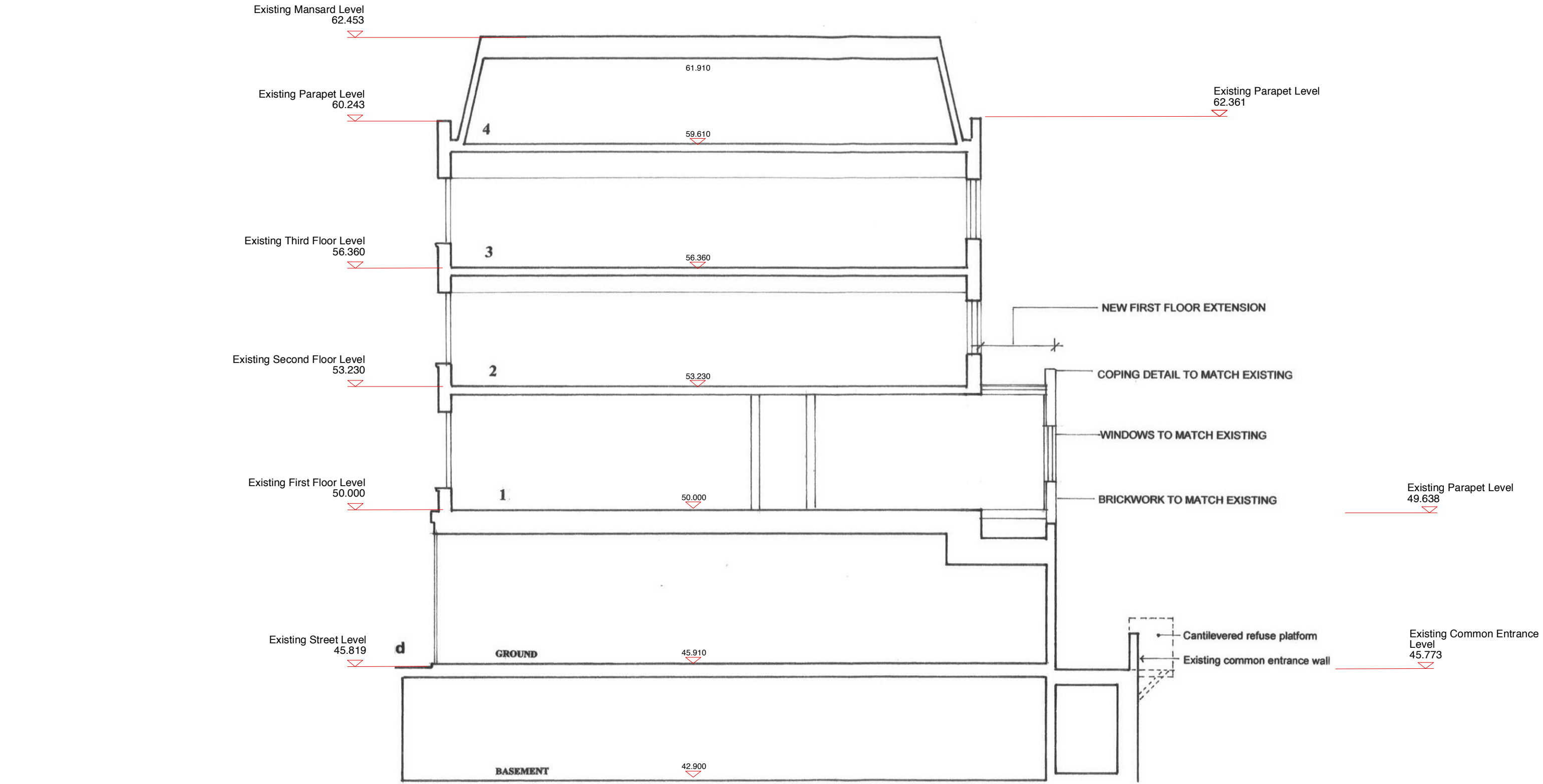
APPROVED SECTION AA Planning Ref: 2010/4614/P
