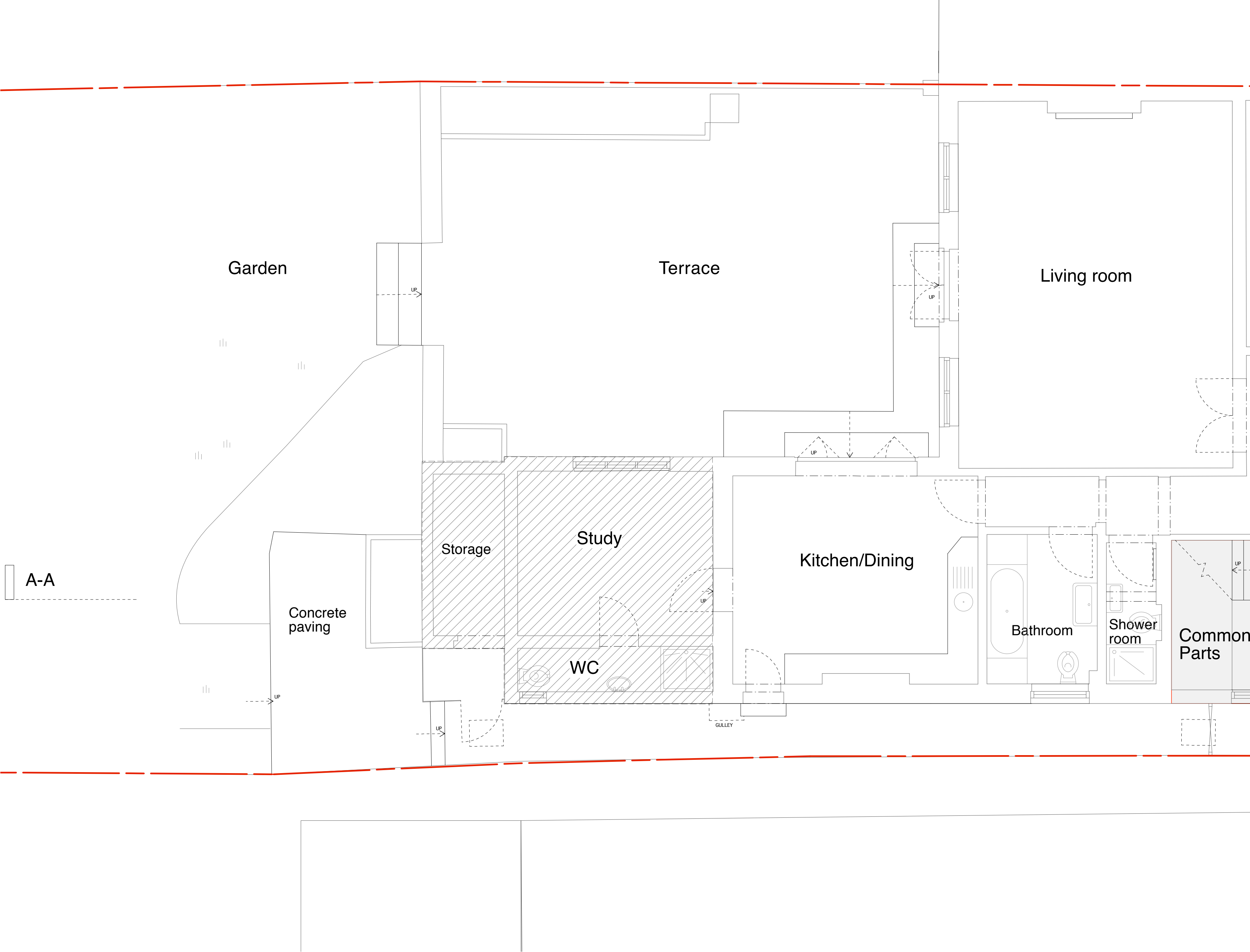
Existing Condition: Ground Floor Plan
