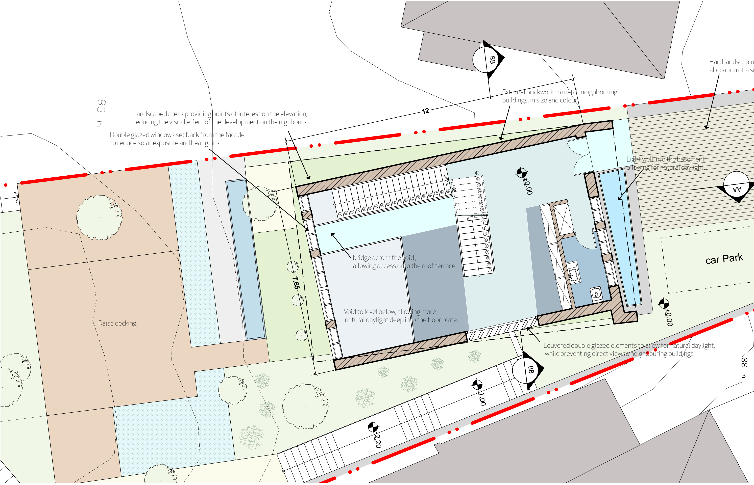
Plan- Ground
