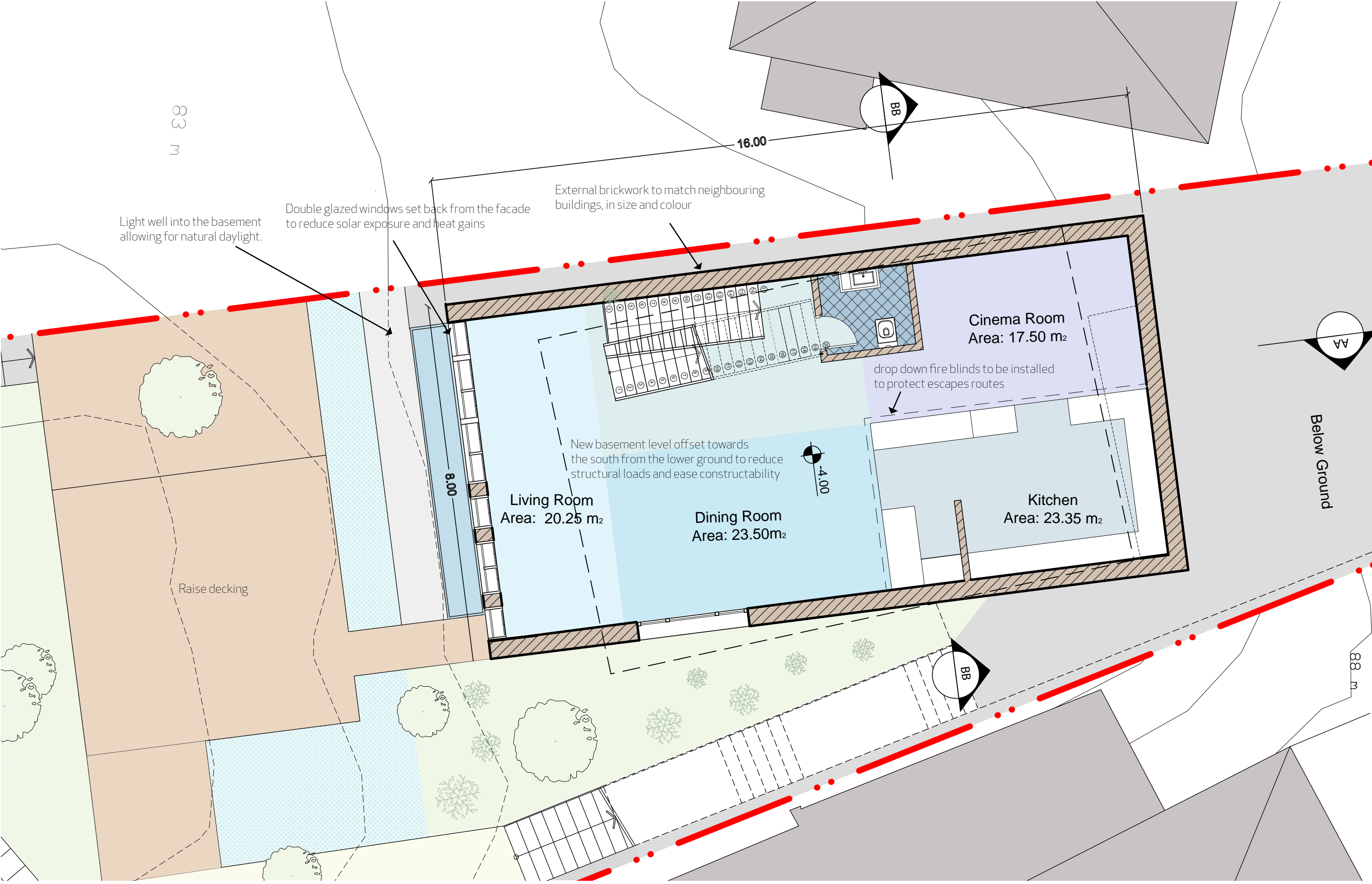
Plan-Lower Ground
