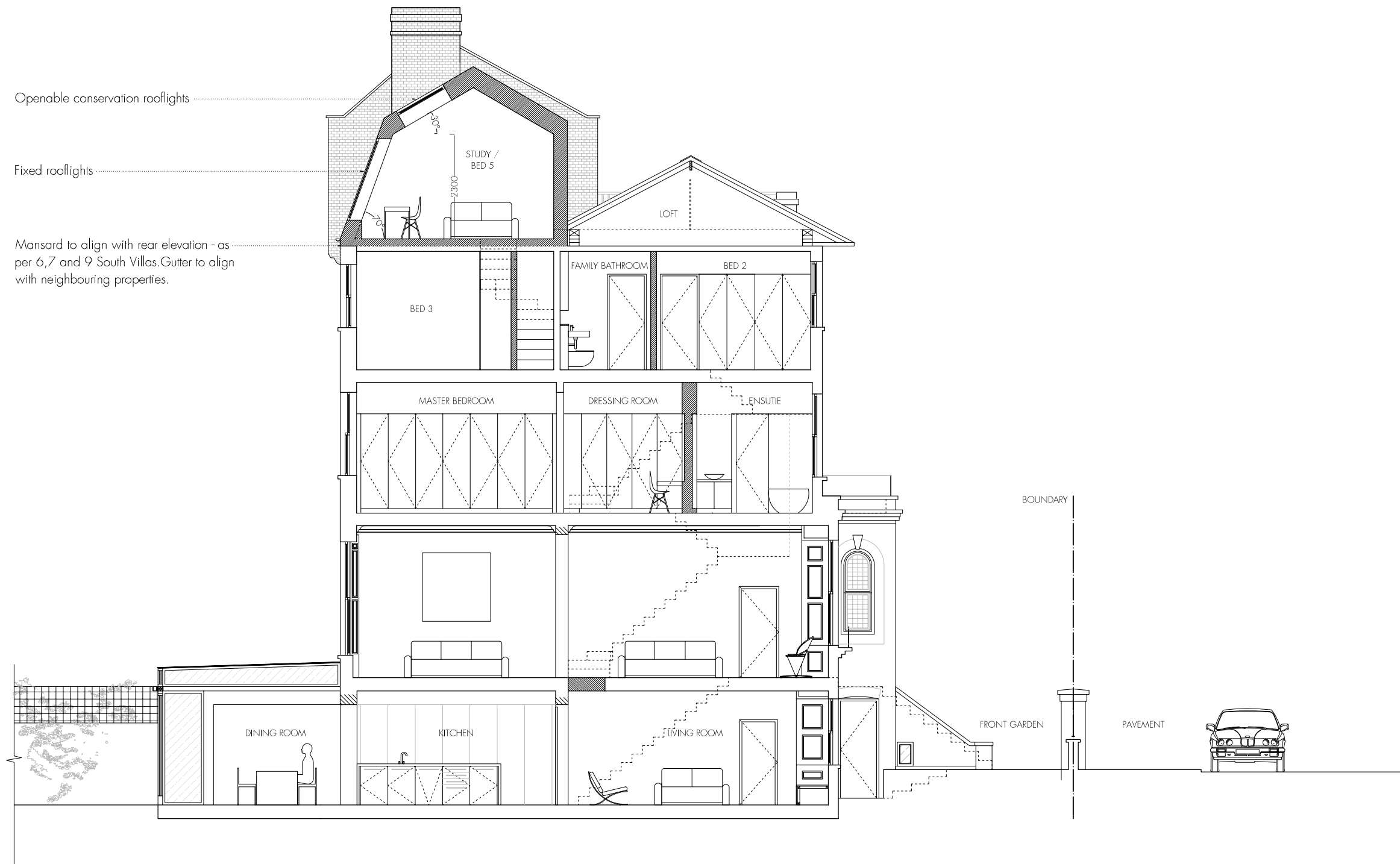
SECTION AA
