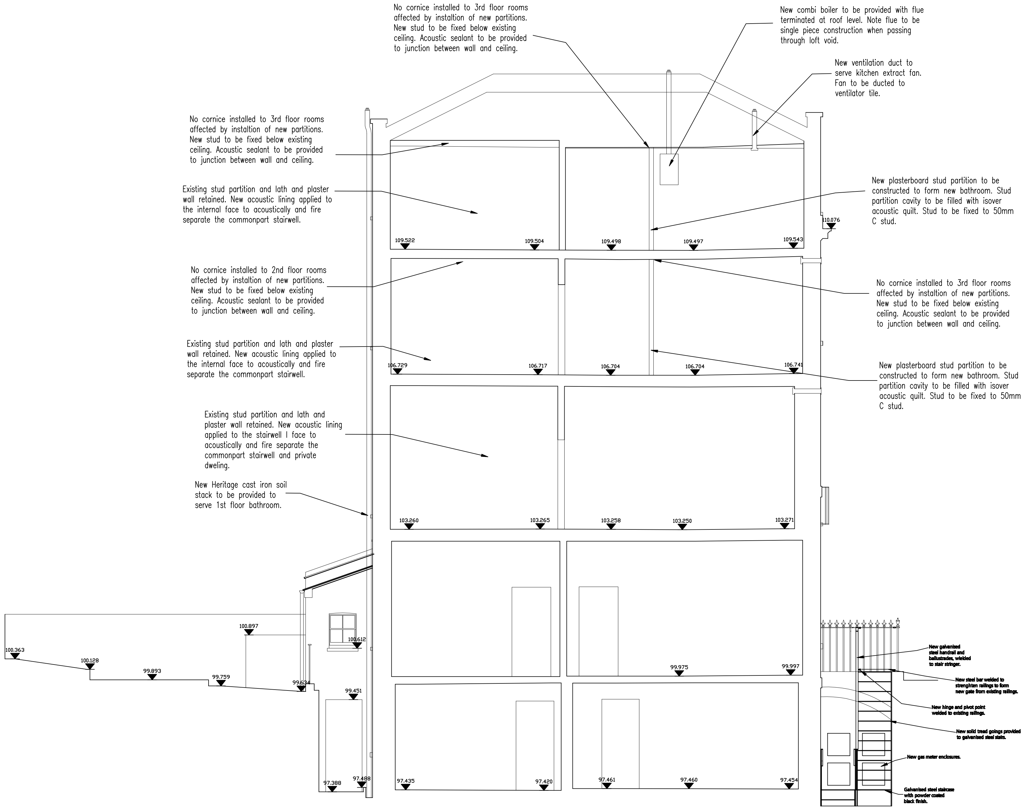
SECTION A - A
