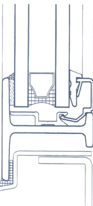
Cill - fixed light
