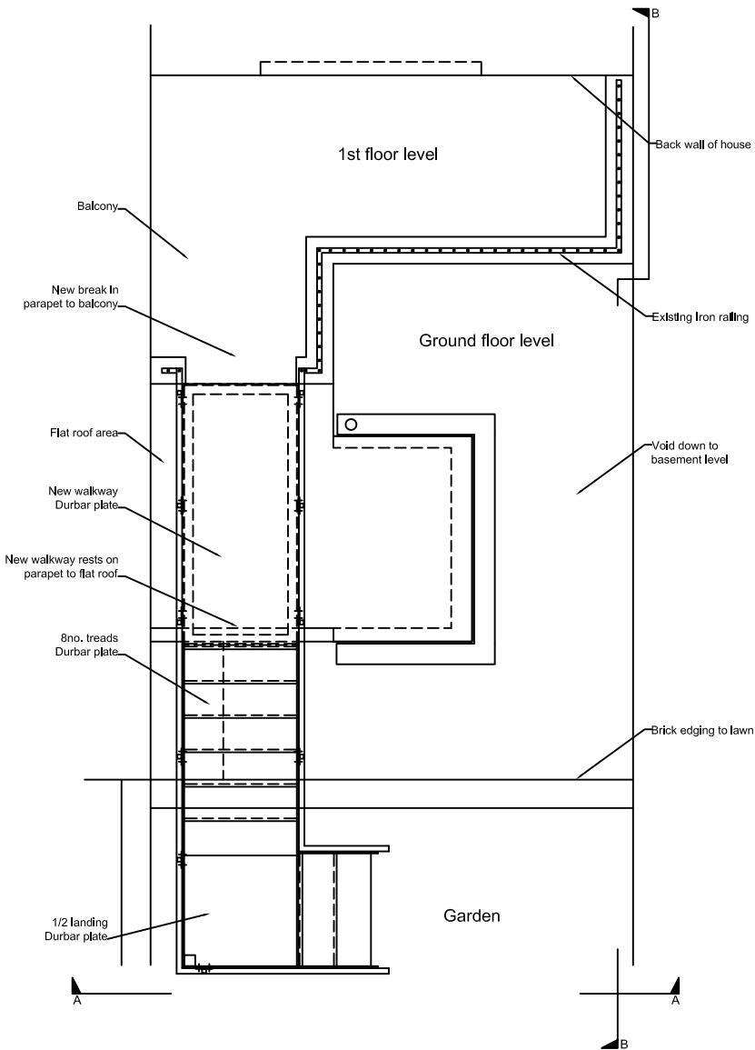
Proposed situation Plan view on rear of house Ground & First floor
