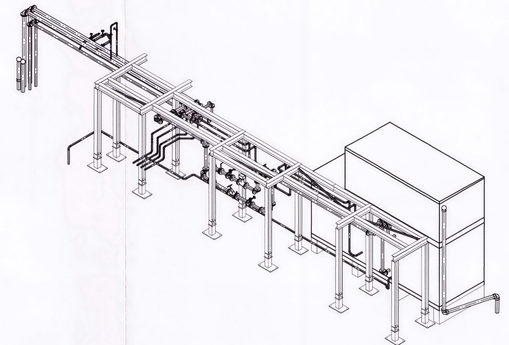
PIPEWORK ISOMETRIC
