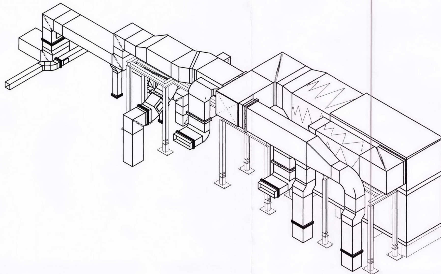
EXTRACT DUCTWORK ISOMETRIC
