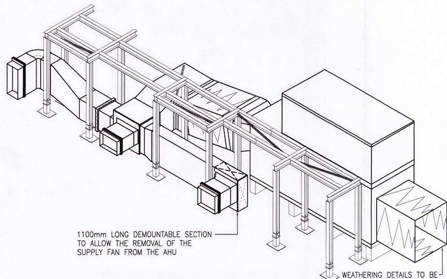
SUPPLY DUCTWORK ISOMETRIC
