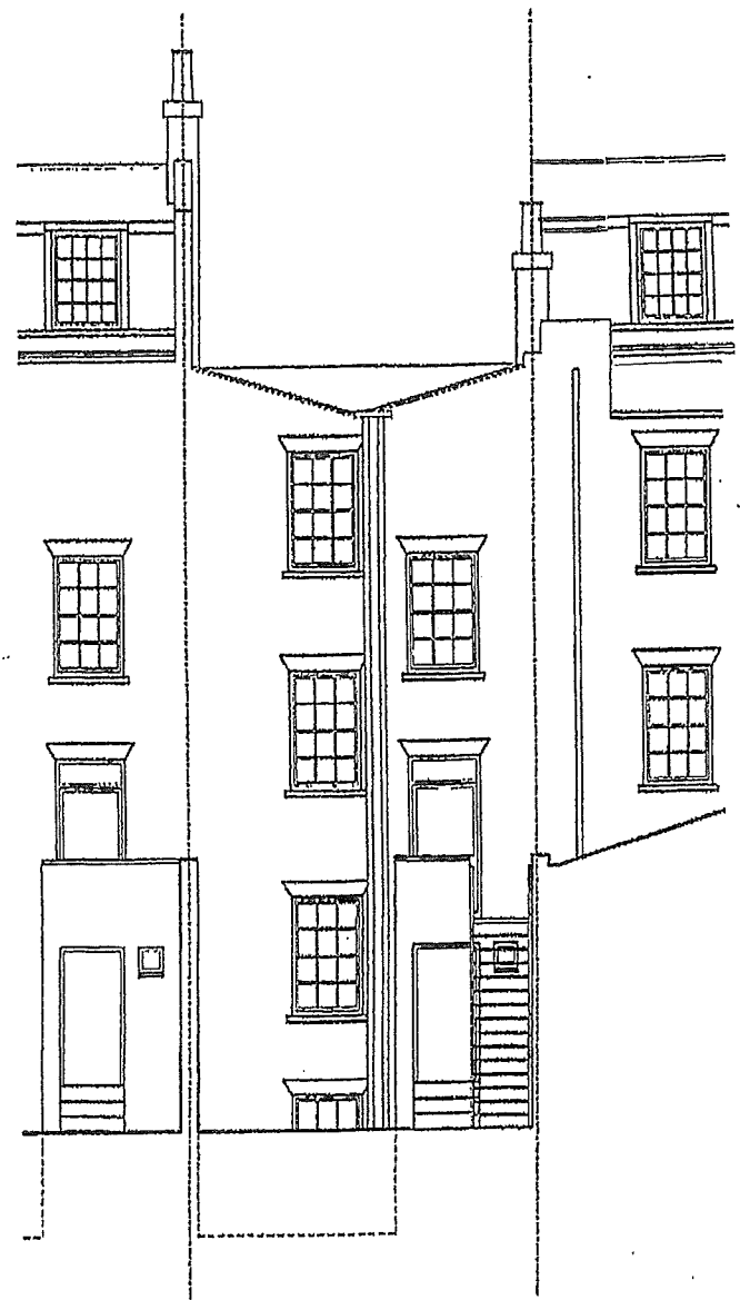
01. REAR ELEVATION - EXISTING
