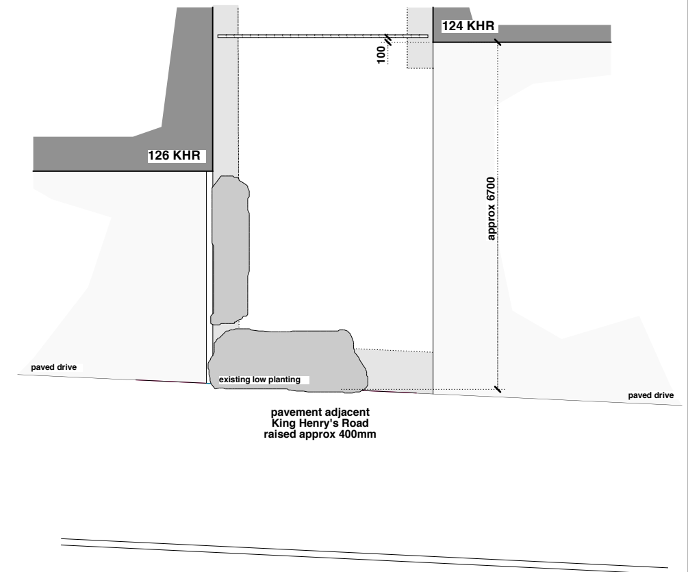
Fence 3 (124-126 KHR)
