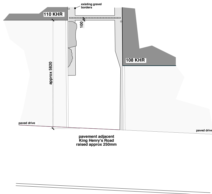
Fence 1 (108-110 KHR)
