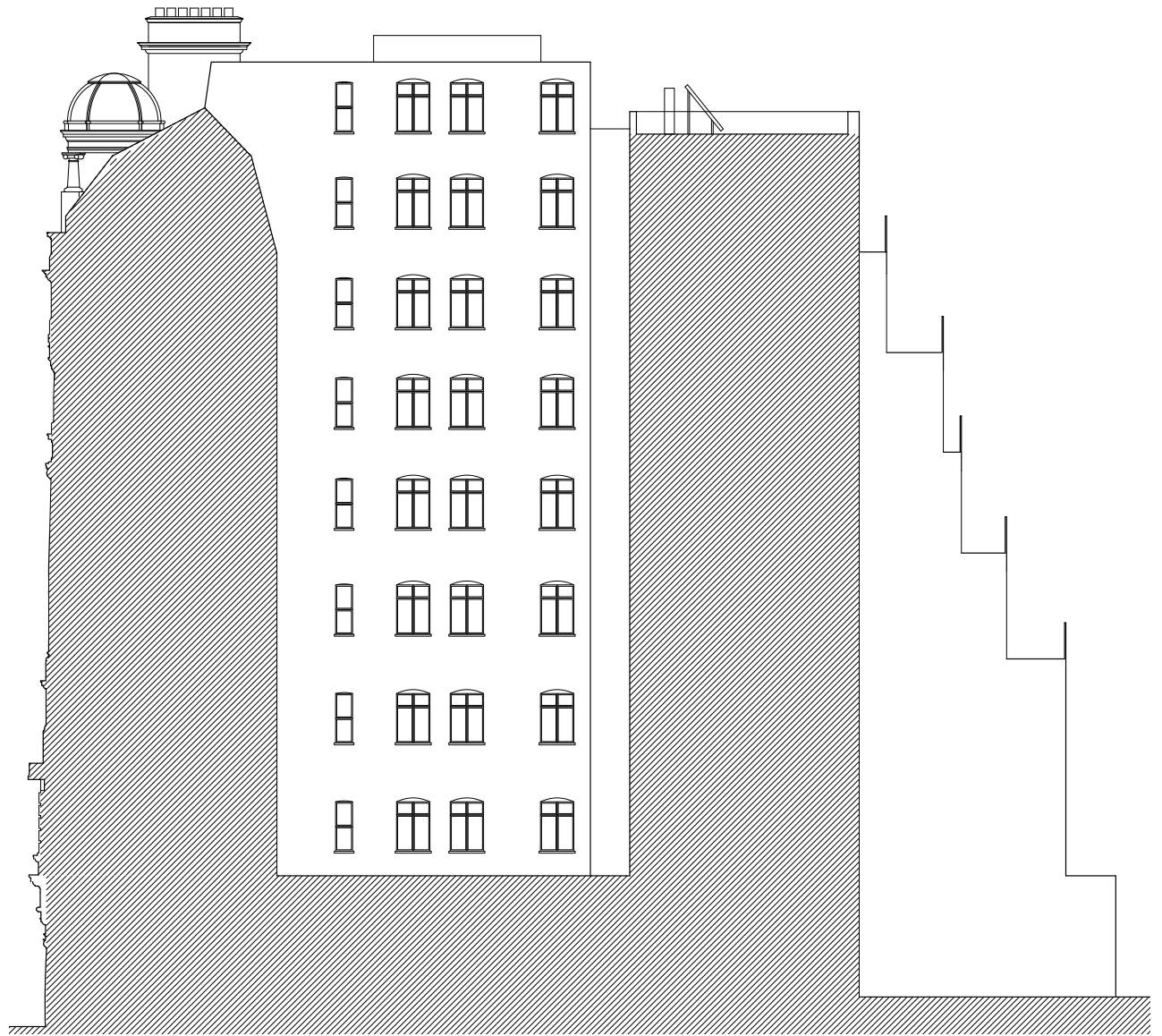
SIDE ELEVATION BB
