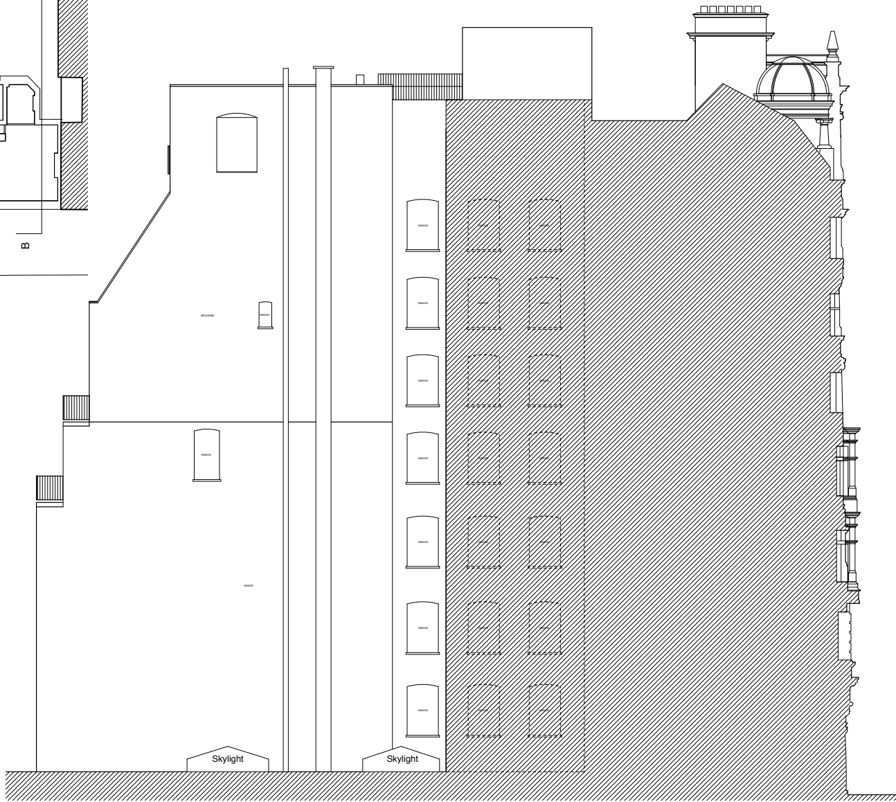
SIDE ELEVATION AA
