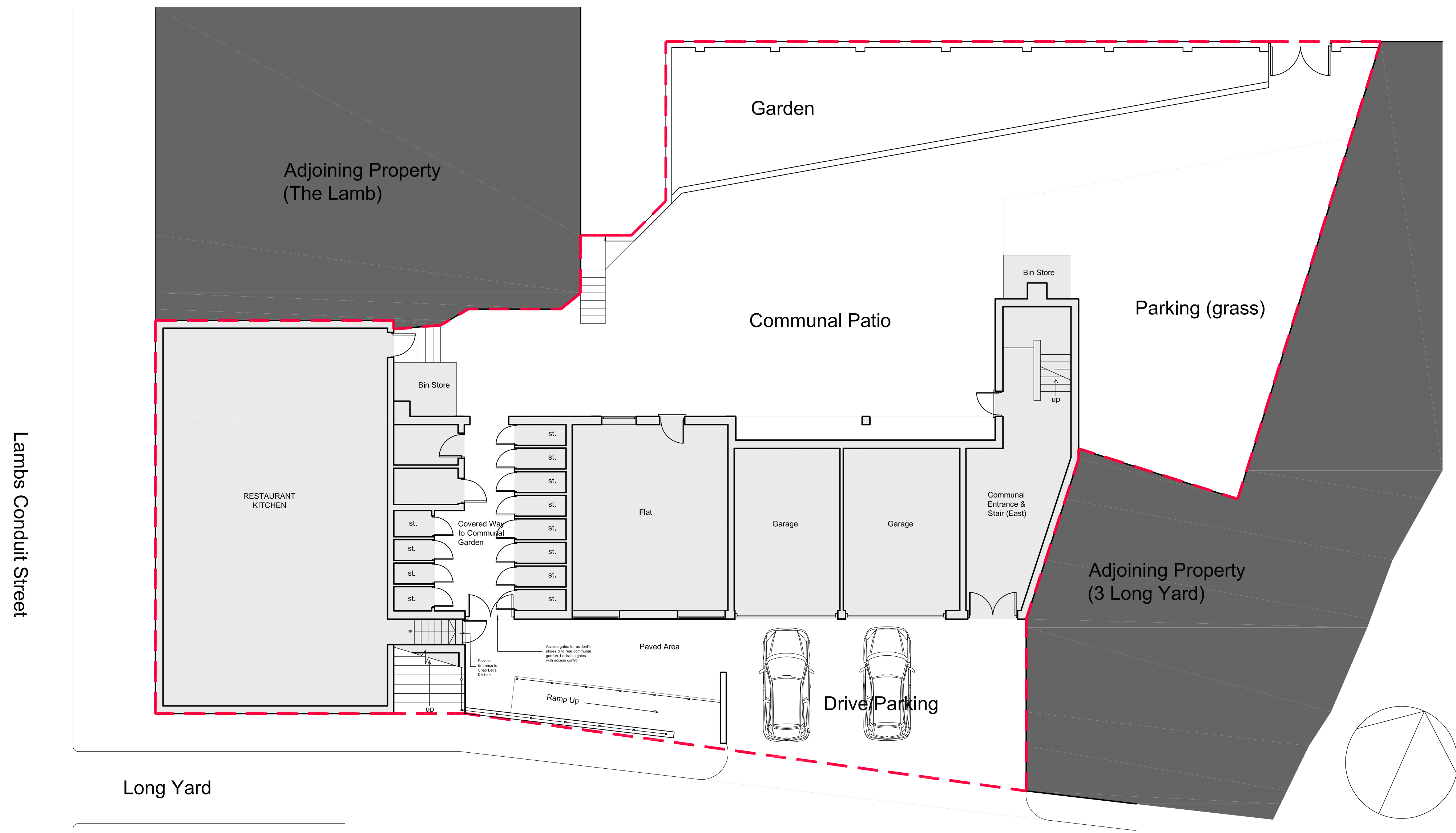
Lower Ground Floor / Site Plan (Existing)
