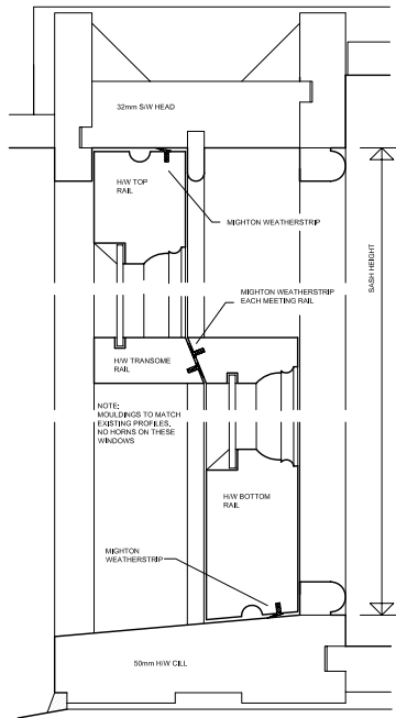
3 | TYPICAL SECTION SASH WINDOW 34 | 1:2
