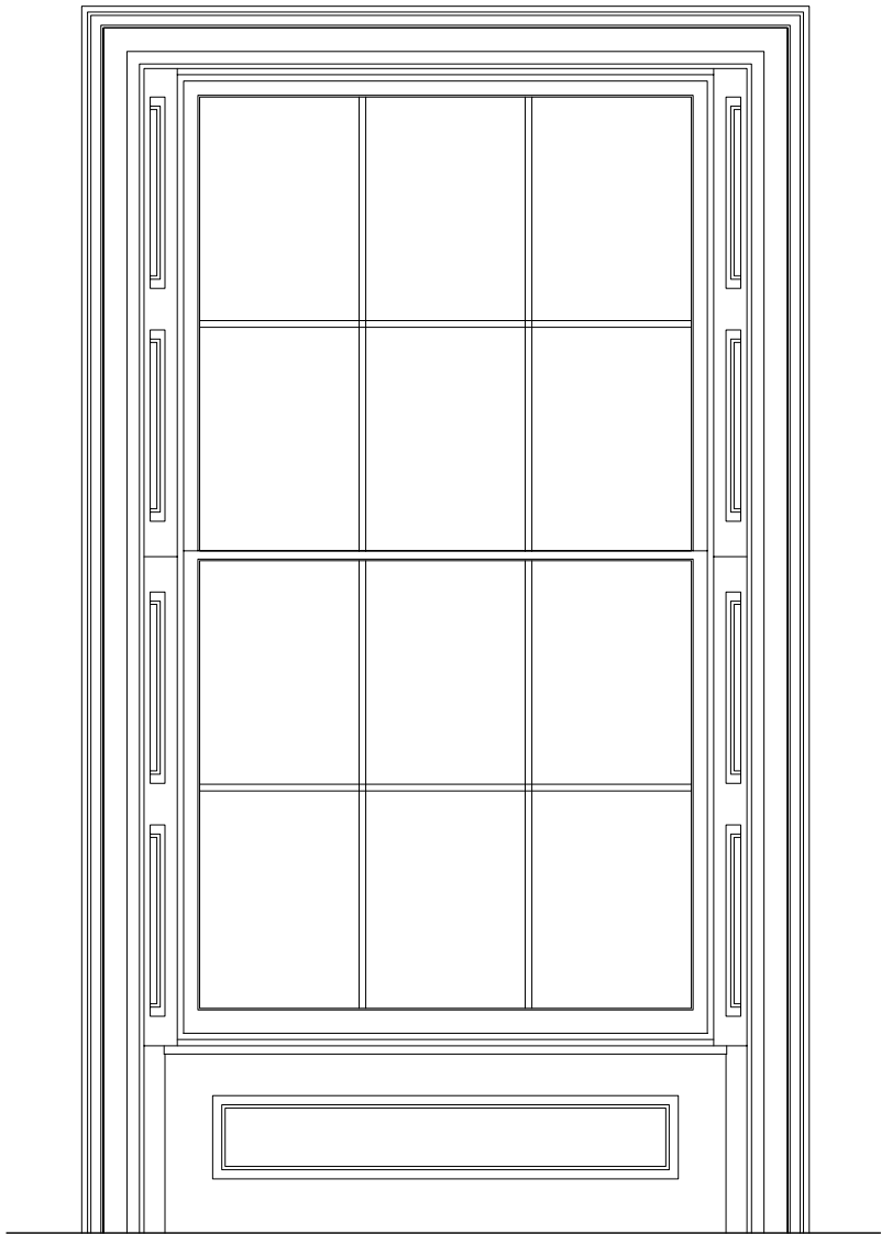
1 | ELEVATION TYPICAL SHUTTER BOXES 35 | 1:10
