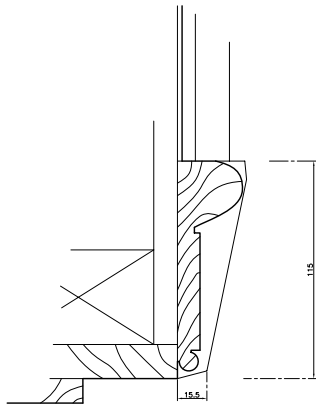
5 | EXISTING ARCHITRAVE TYPICAL PLAN 30 | 1:2
