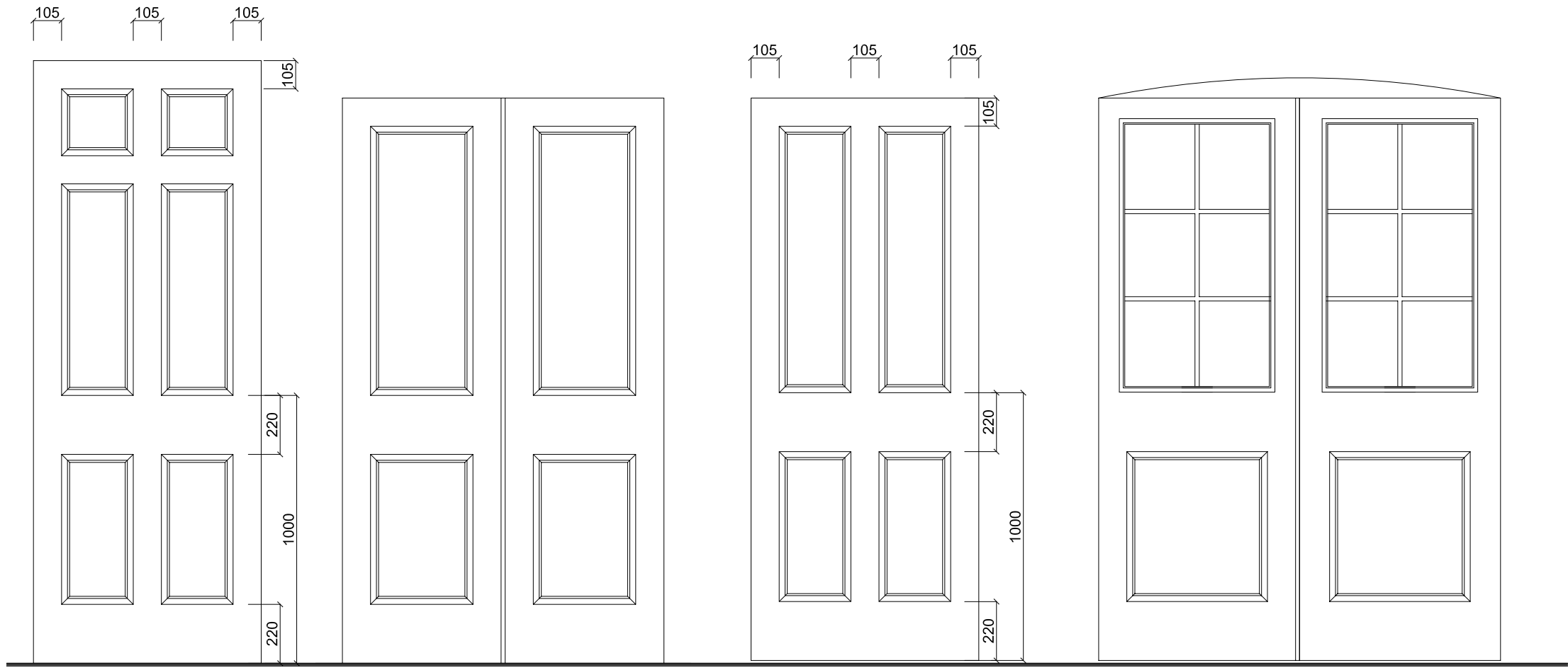
1 6 PANEL DOOR ELEVATION 2 4 PANEL PAIR OF DOORS ELEVATION 3 TYPICAL 4 PANEL DOOR ELEVATION 4 GUN STOCK DOOR AND FIXED PANEL (basement under entrance steps) 31 1:10 31 1:10 31 1:10 31 1:10
