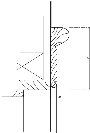
3 | EXISTING DOOR HEAD DETAIL 30 | 1:2
