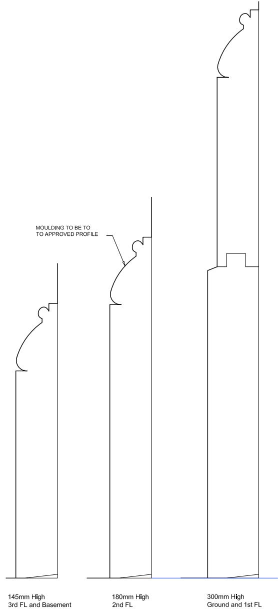
5 TYPICAL SKIRTINGS 31 1:1
