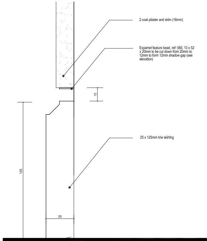
4 BASEMENT SKIRTING DETAIL (NEW AREAS) 32 1:2
