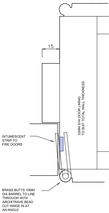
6 TYPICAL DOOR LINING 31 1:1
