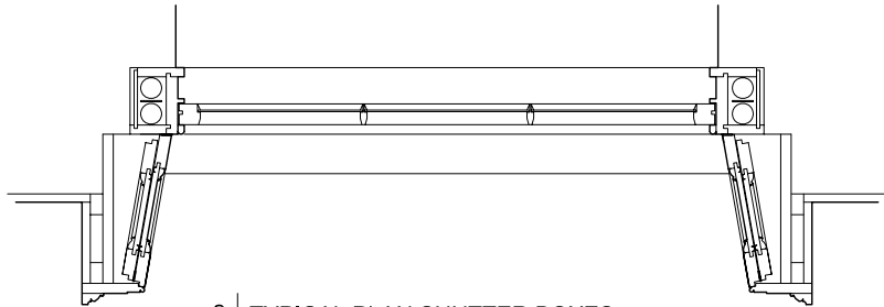
2 | TYPICAL PLAN SHUTTER BOXES 35 | 1:10
