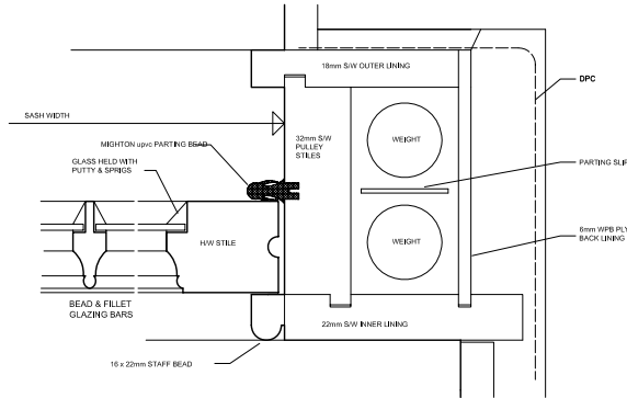
2 | TYPICAL PLAN OF SASH BOX 34 | 1:2
