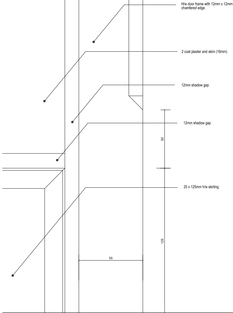
5 PART ELEVATION BASEMENT DOOR FRAMES (NEW AREAS) 32 1:2
