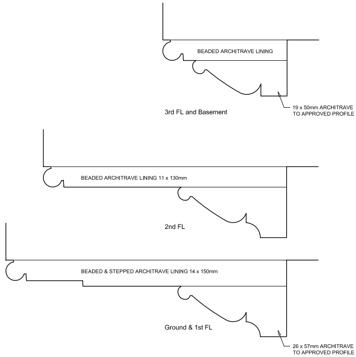
7 TYPICAL ARCHITRAVES 31 1:1
