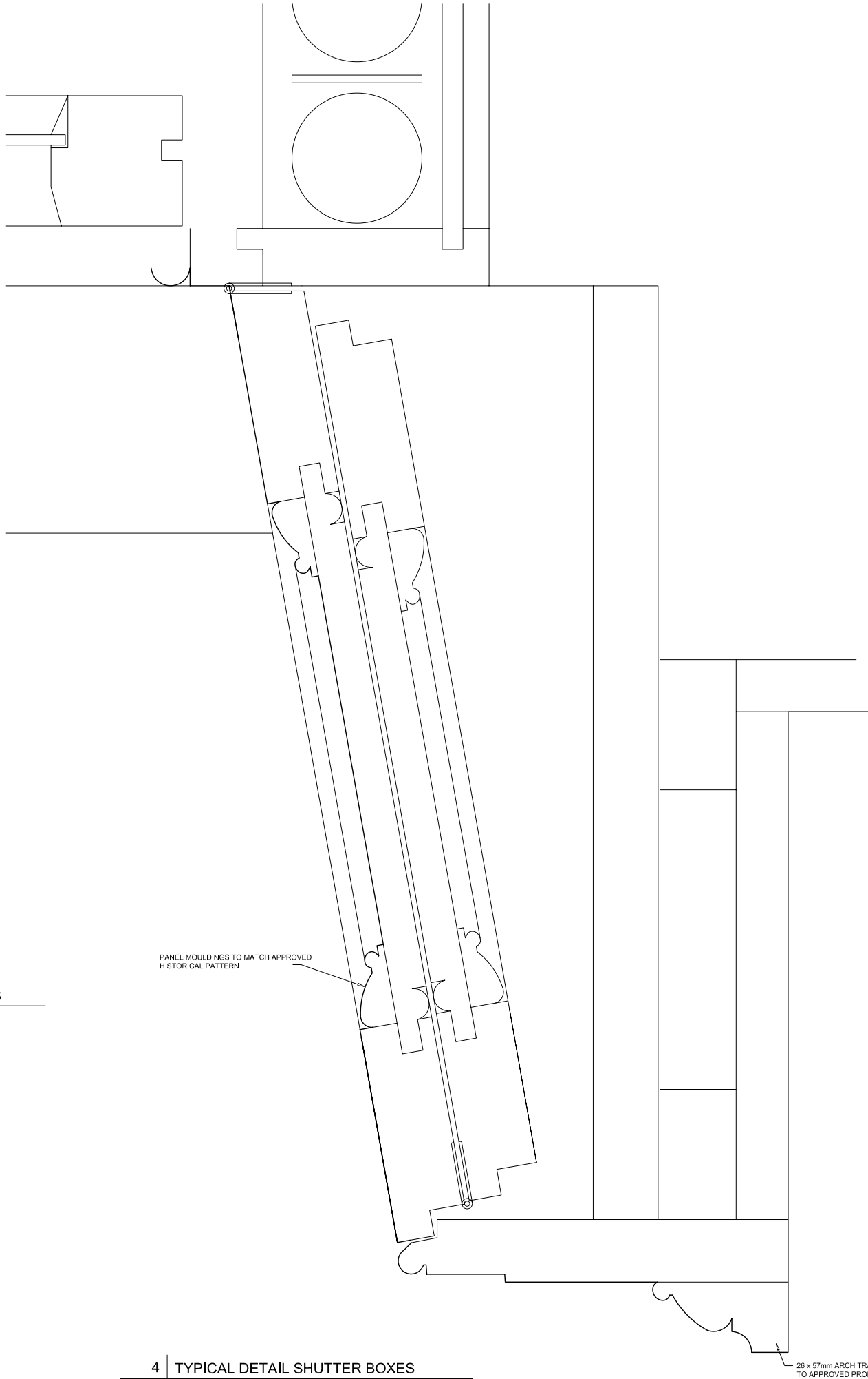
4 | TYPICAL DETAIL SHUTTER BOXES 35 | 1:1
