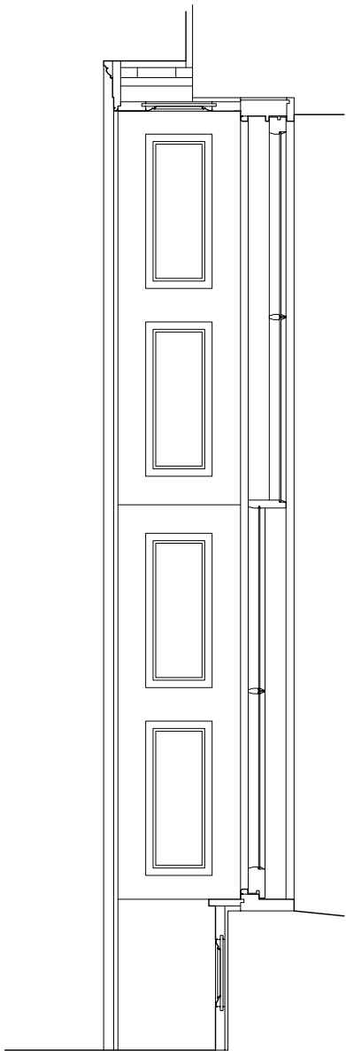
3 | TYPICAL SECTION SHUTTER BOXES 35 | 1:10
