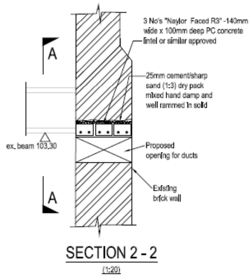
Engineers drawing of new opening through wall
