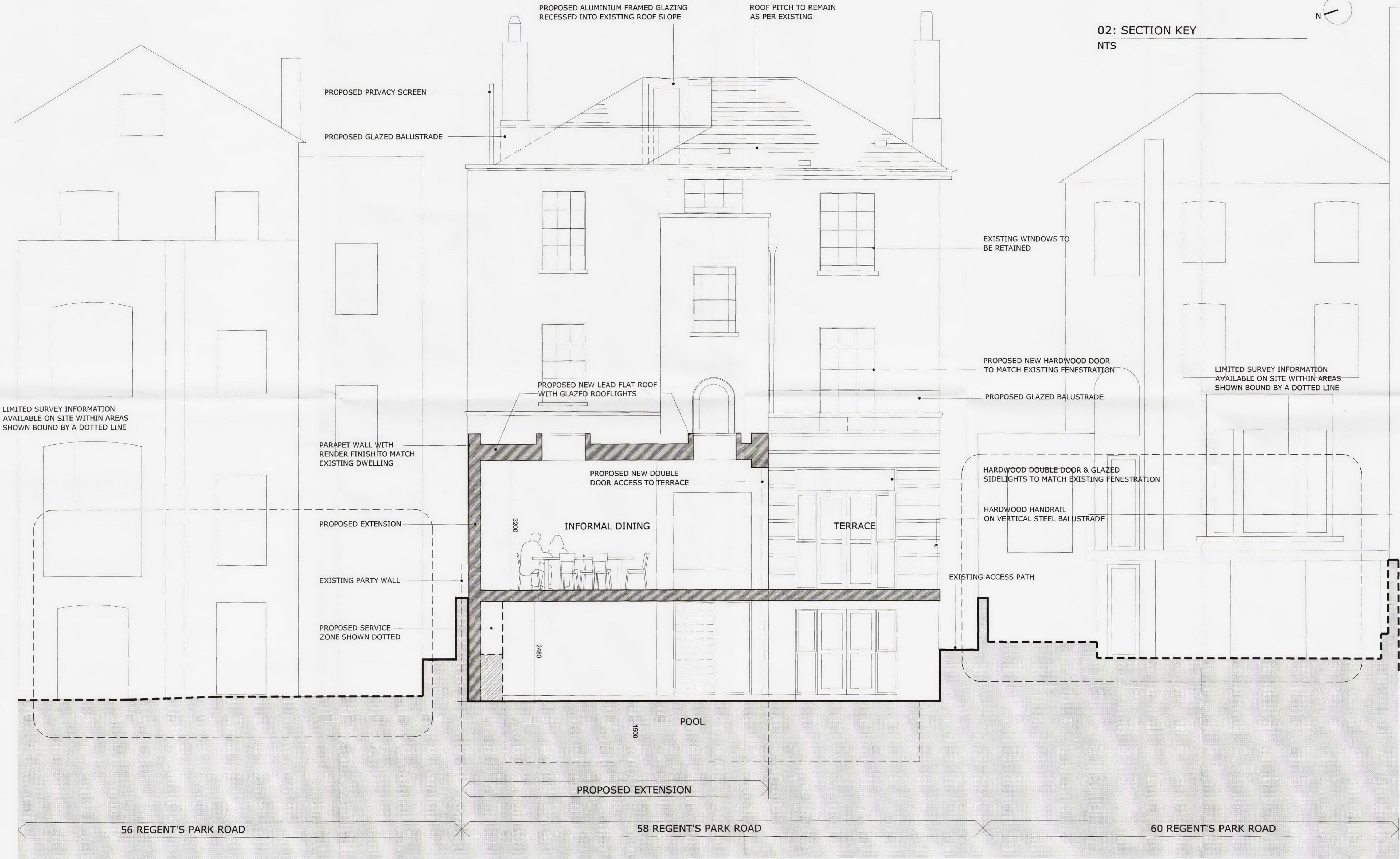
01: SECTION B-B SCALE 1:50 at A1
