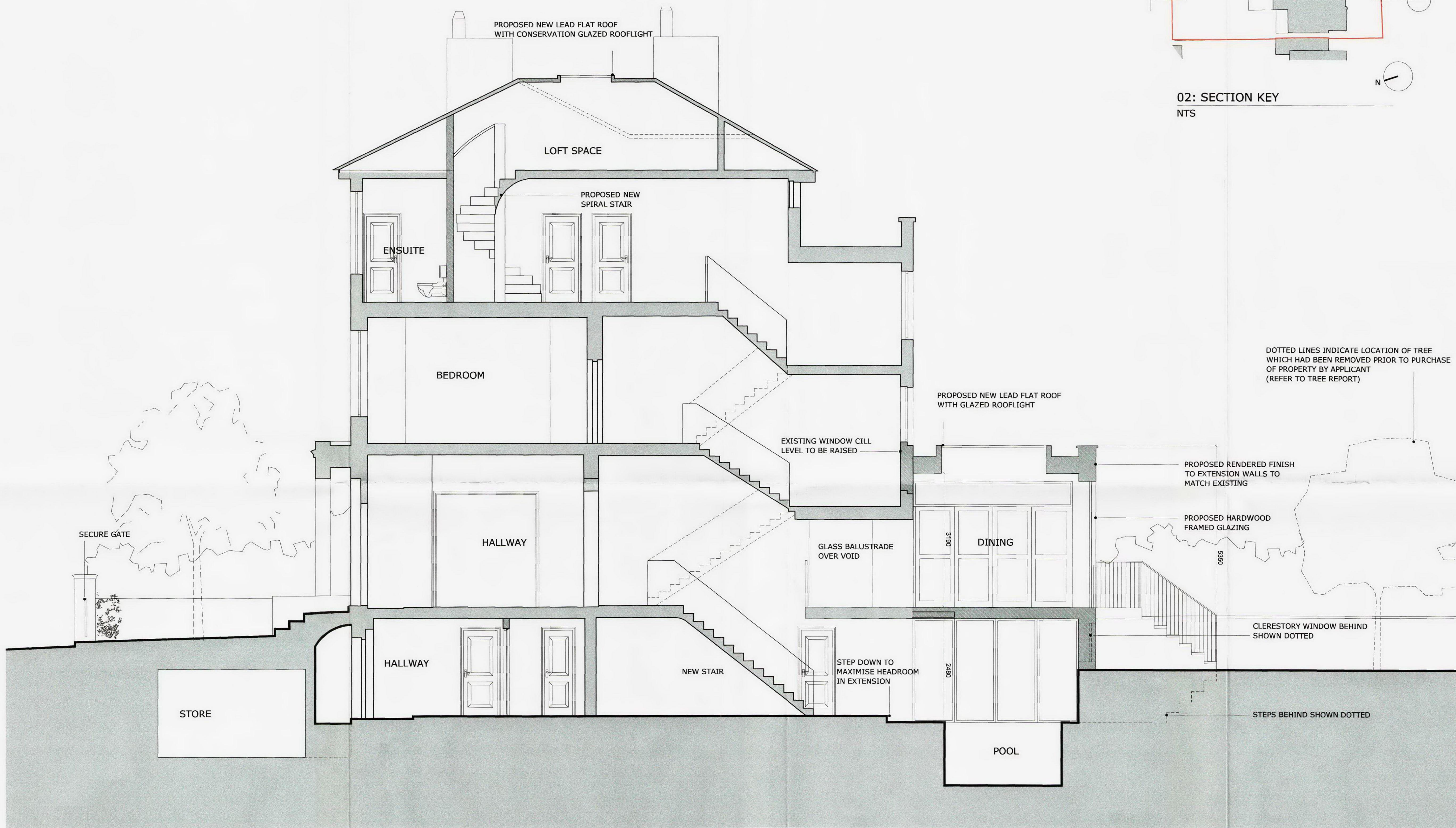
01: CROSS SECTION A-A SCALE 1:50 at A1
