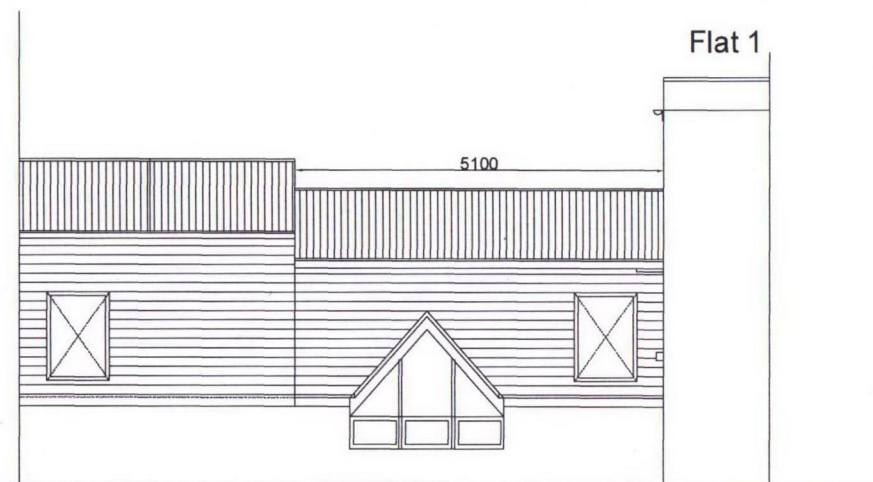
LHS Elevation 1:100
