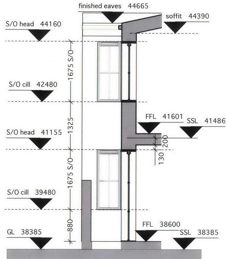
SECTION A56-2 TO WESTERN BOUNDARY
