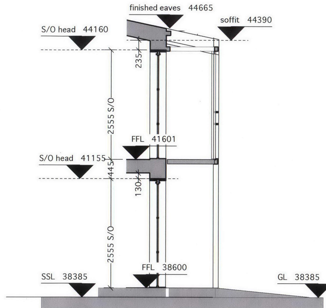
SECTION A56-2 TO COURTYARD
