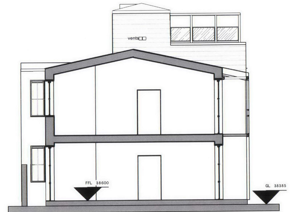
ELEVATION A56-3 OUTSIDE ROOF GARDEN & INSIDE ACCESS BALCONY
