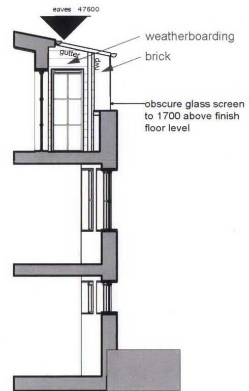
ELEVATION A52-3 OUTSIDE TERRACE - UNIT 8
