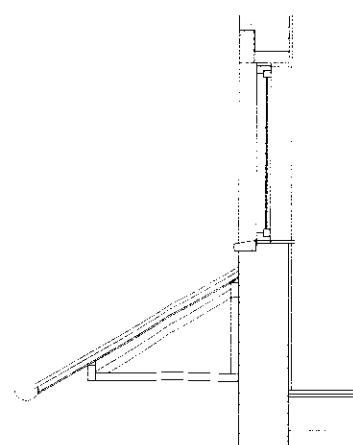
W3 Existing Section
