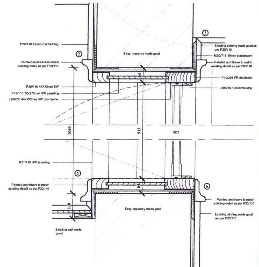
PLAN DETAIL 1-5
