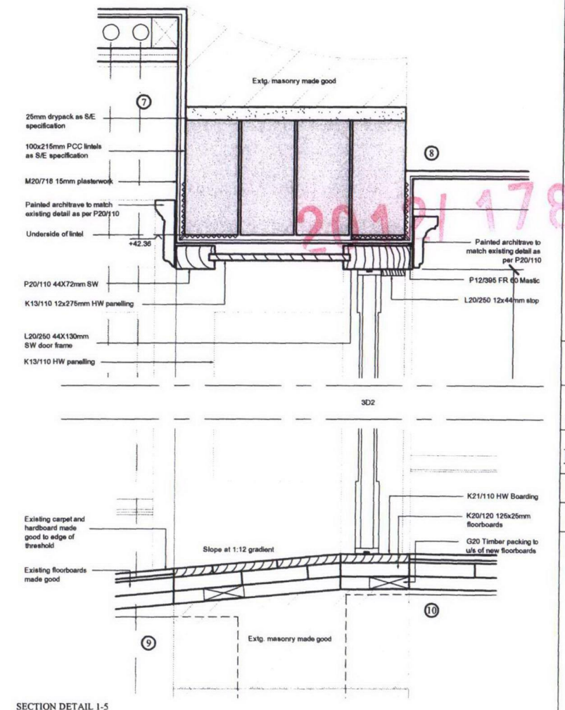
SECTION DETAIL 1-5
