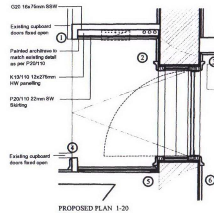
PROPOSED PLAN 1-20
