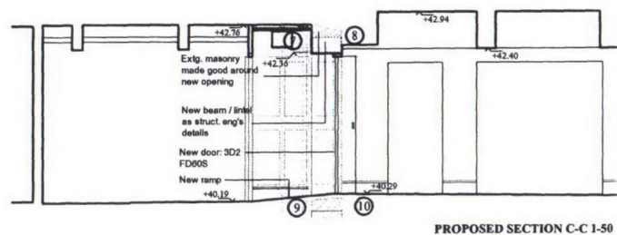
PROPOSED SECTION C-C 1-50
