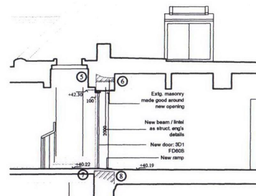
PROPOSED SECTION C-C 1-50
