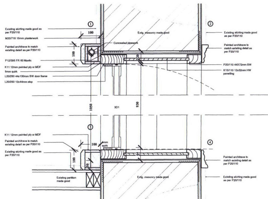
PLAN DETAIL 1-5
