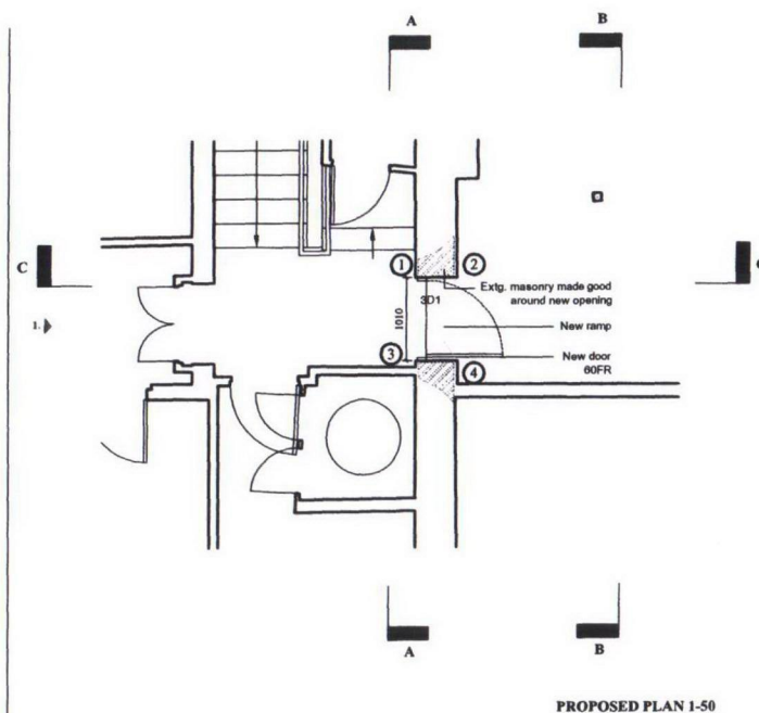
PROPOSED PLAN 1-50
