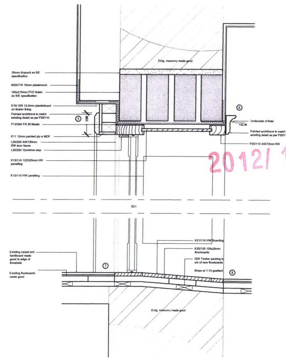
SECTION DETAIL 1-5
