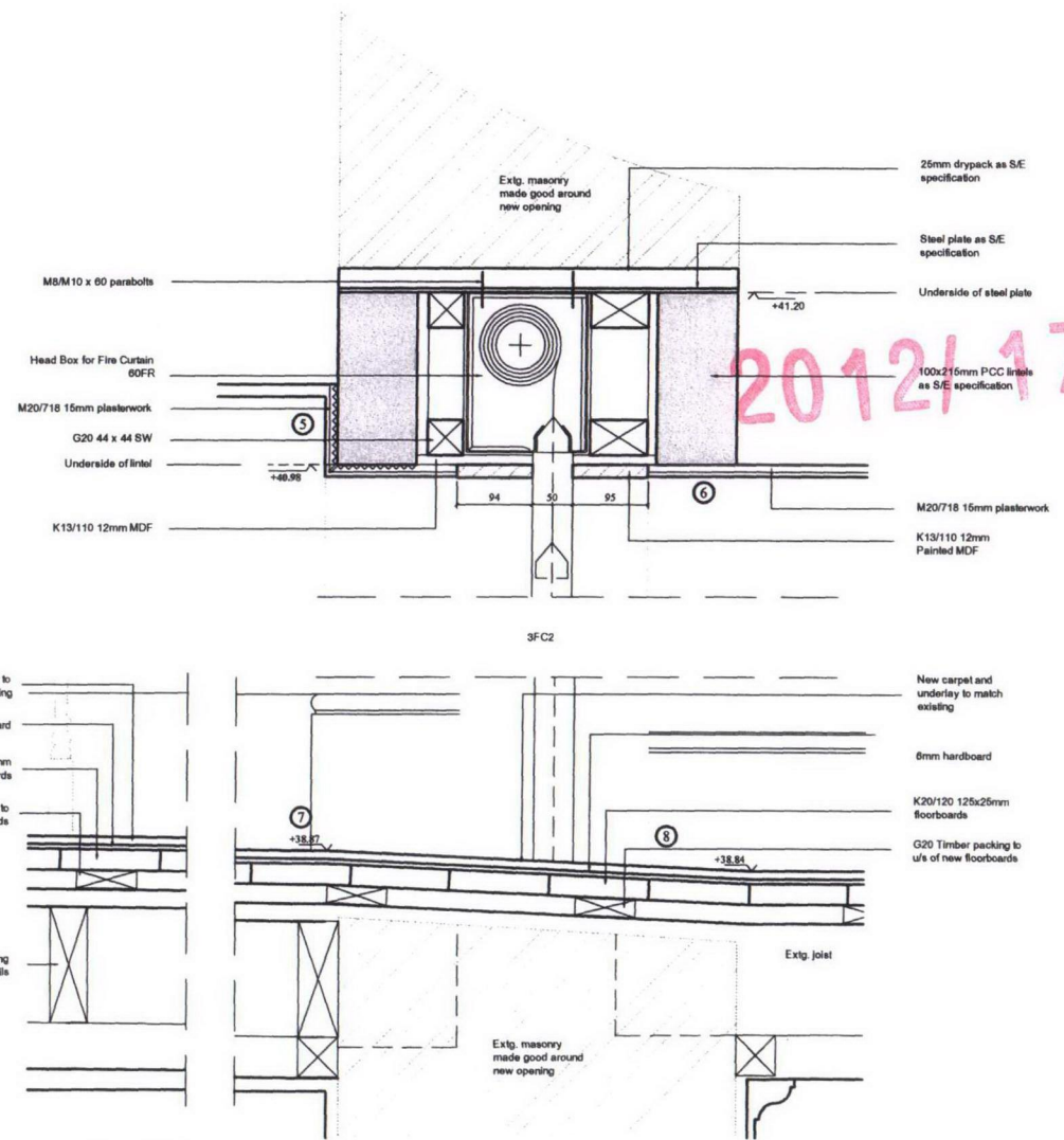
SECTION DETAIL 1-5
