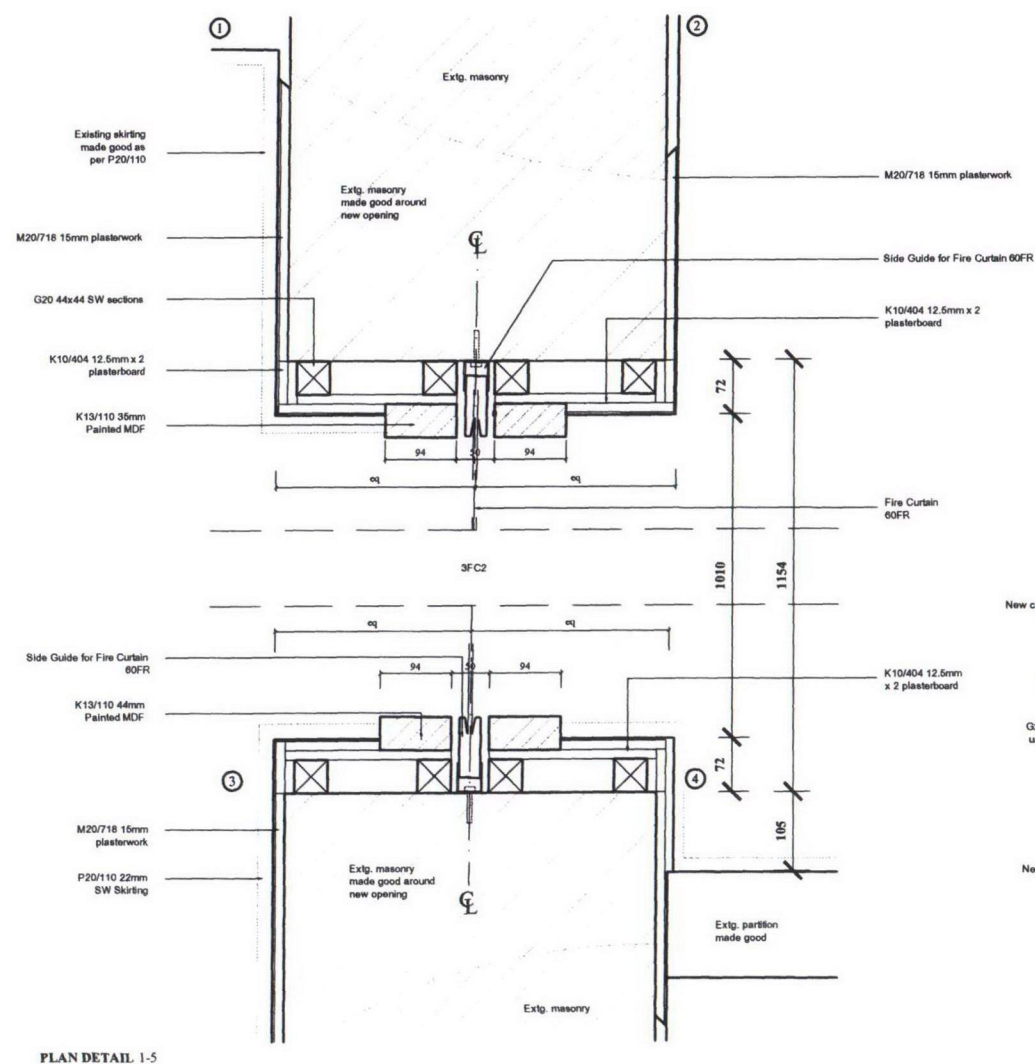
PLAN DETAIL 1-5
