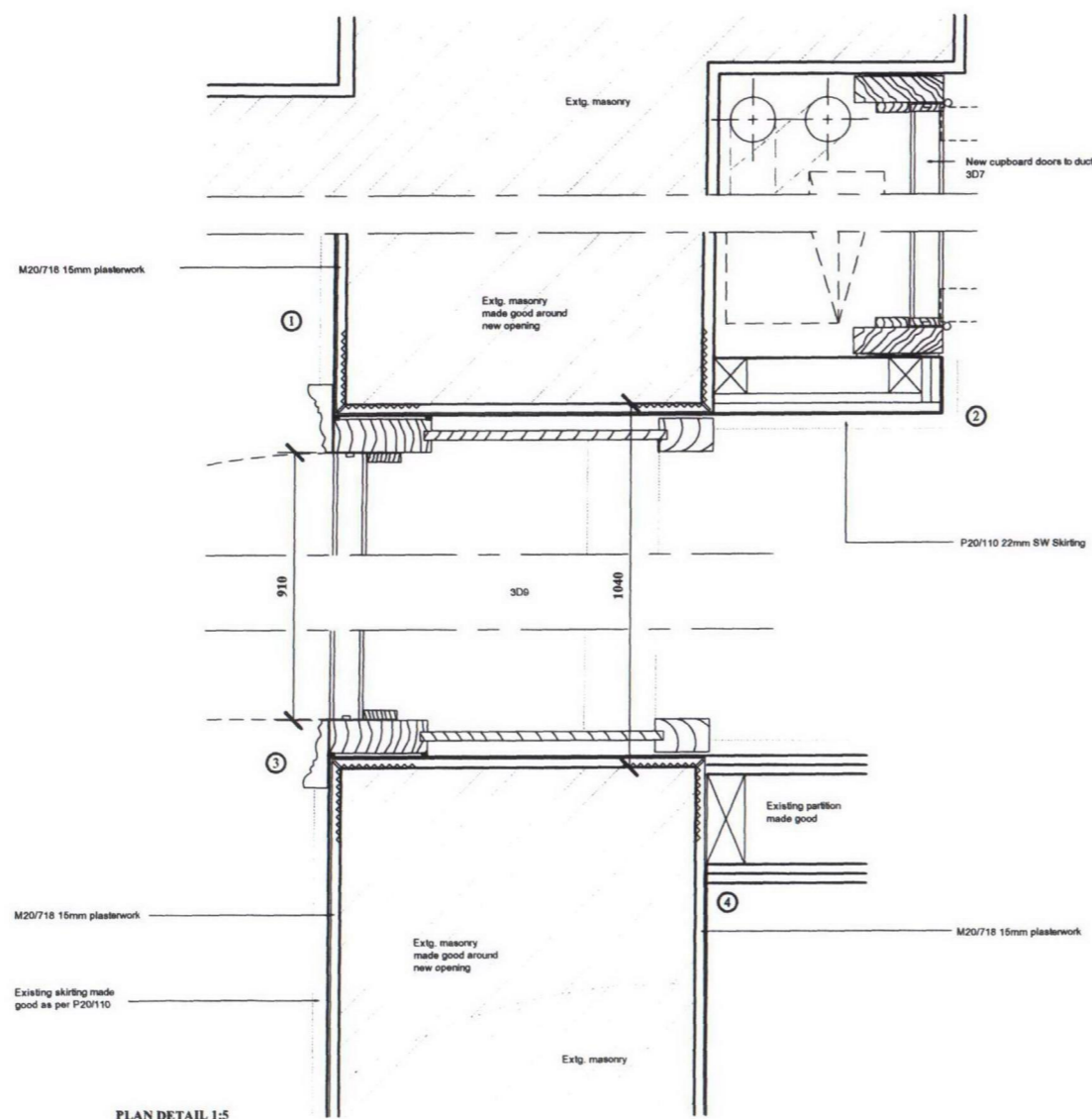
PLAN DETAIL 1:5
