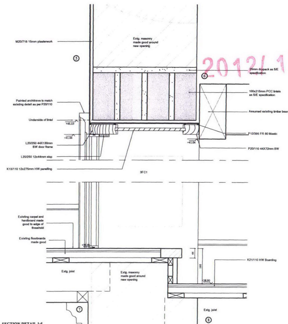
SECTION DETAIL 1:5
