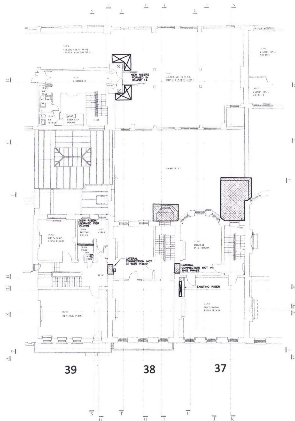
FIRST FLOOR DEMOLITIONS, PRIMARY BUILDERSWORK & REMOVALS (SEE ARCHITECT'S DRAWINGS FOR DETAILS)
