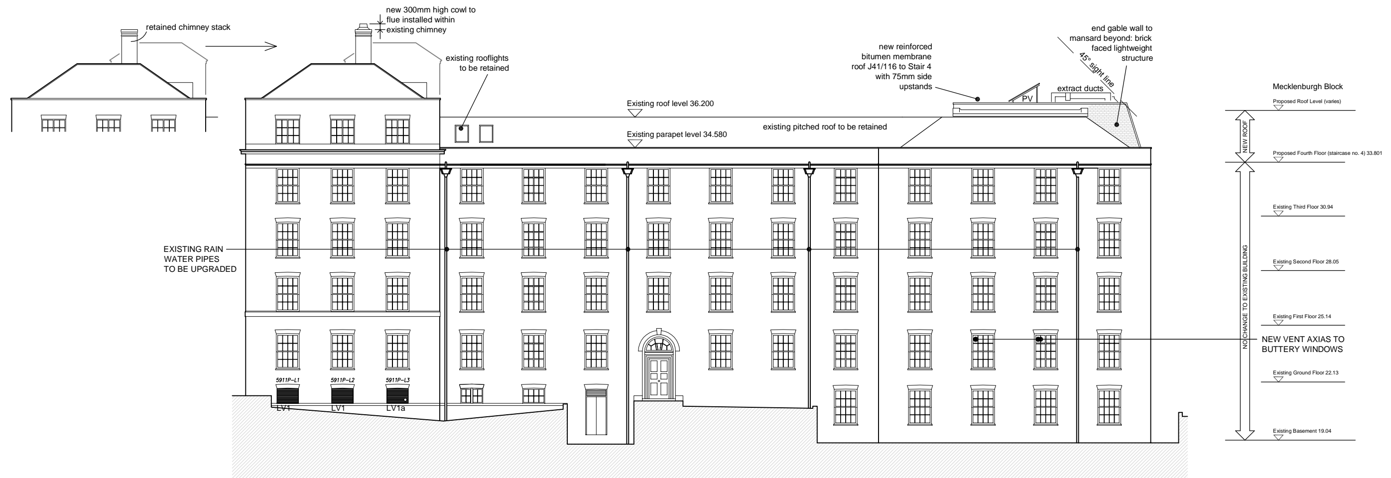
ELEVATION 5 - FRONT OF MECKLENBURGH BLOCK (EAST-FACING) SCALE: 1:100
