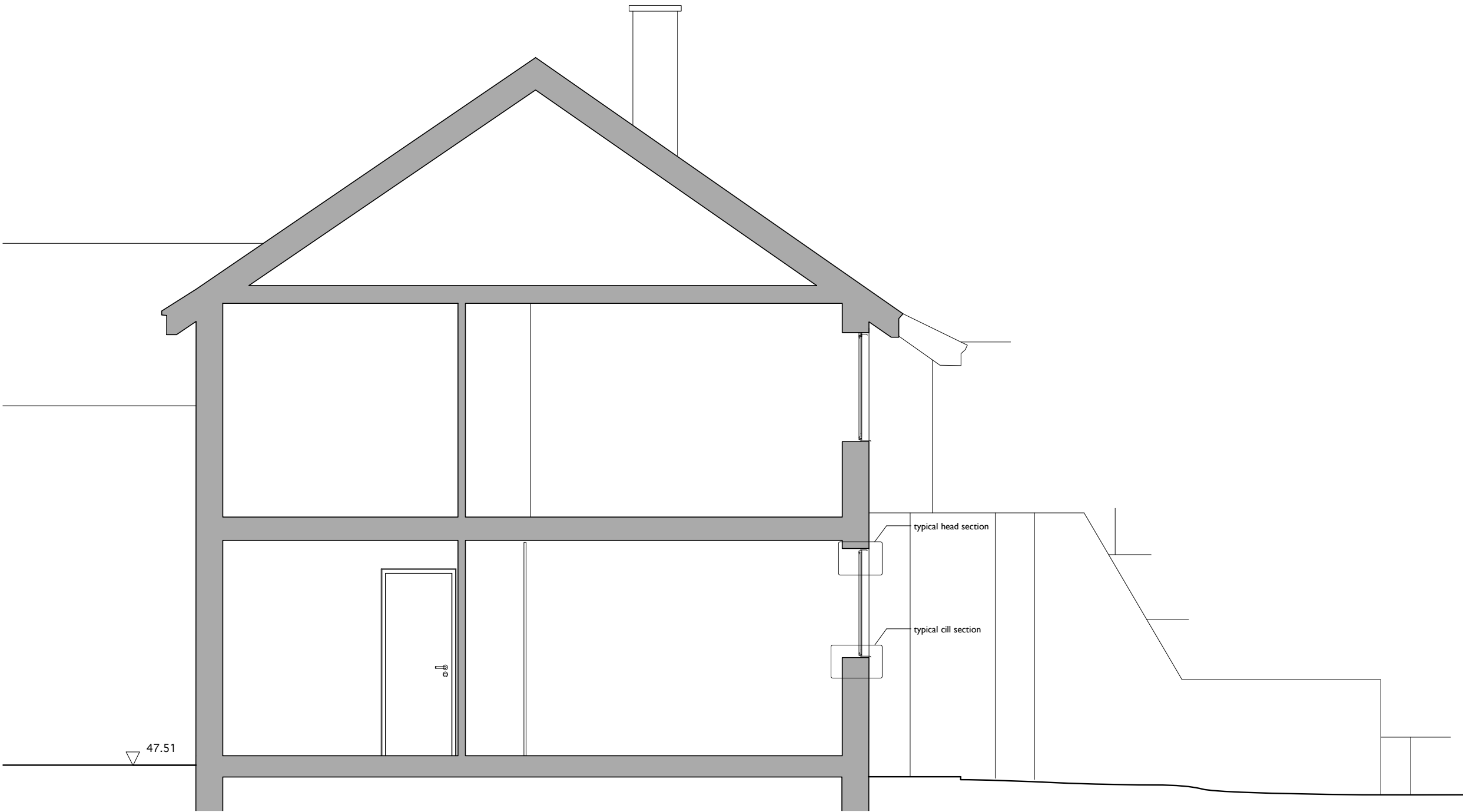
Existing Section B - B @ 1:50
