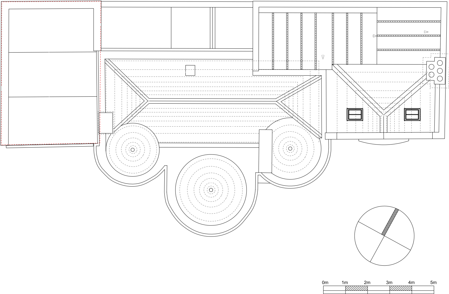
Roof Plan
